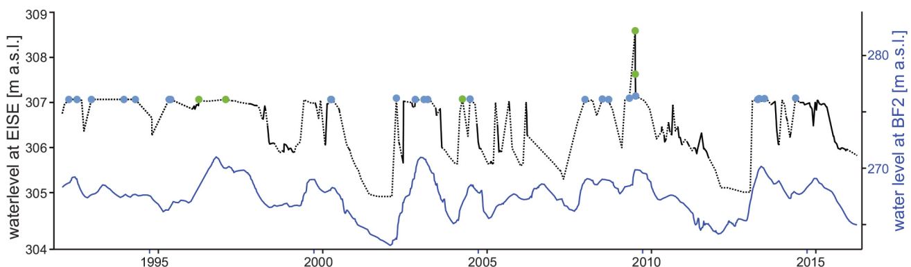
Figure 5: Water level of the spring at EISE between 1992 and 2015. Blue dots indicate overflow into the Lehmabad, green dots indicate flooding of the Lehmabad, dotted lines indicate a sampling interval of more than 21 days: the full line indicates sampling intervals of 21 days or less. The level in well BF2 (blue graph) shows the highest correlation if a delay of 14 weeks is applied as in the figure ( R increased from 0.68 to 0.78).
