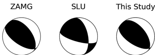
Figure 7: Fault plane solutions. Left: 323^\circ/41^\circ/105^\circ from Zentralanstalt für Meteorologie und Geodynamik (ZAMG) based on first P-, SH-, and SV-arrival polarities (Freudenthaler, pers. comm.). Center: 348^\circ/46^\circ/144^\circ from Saint Louis University Earthquake Center based on waveform fitting with synthetics using only permanent stations that are preferentially distributed towards North and South (Saint Louis University, 2016). Right: 317^\circ/40^\circ/101^\circ from this study.
