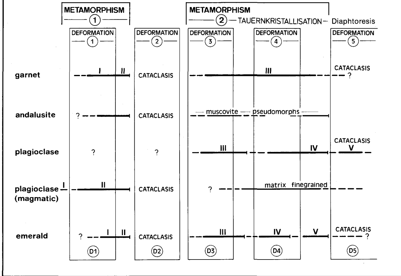
Fig. 3: Crystallization – deformation diagram for garnet, andalusite, plagioclase and emerald in the metapelites and adjacent metavolcanic rocks of the Habachformation southeast of the “Habachzunge” (Untersulzbachtal, Habachtal, Hollersbachtal) (modified after GRUNDMANN & MORTEANI, 1982).
