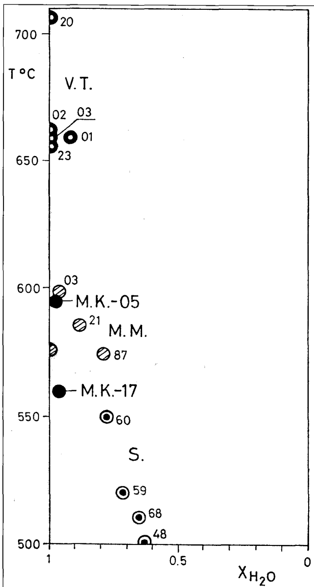
Text-Fig. 8. ◁◁ Composition of metamorphic fluid ( X_{H_2O} ) released by dehydration reactions during metamorphic culmination. Calculated according to equilibrium reaction Par + Qtz = Ab + Sil + H_2O using FERRY'S (1980) thermodynamic data and LANG & RICE (1985) activity formulation for paragonite.
