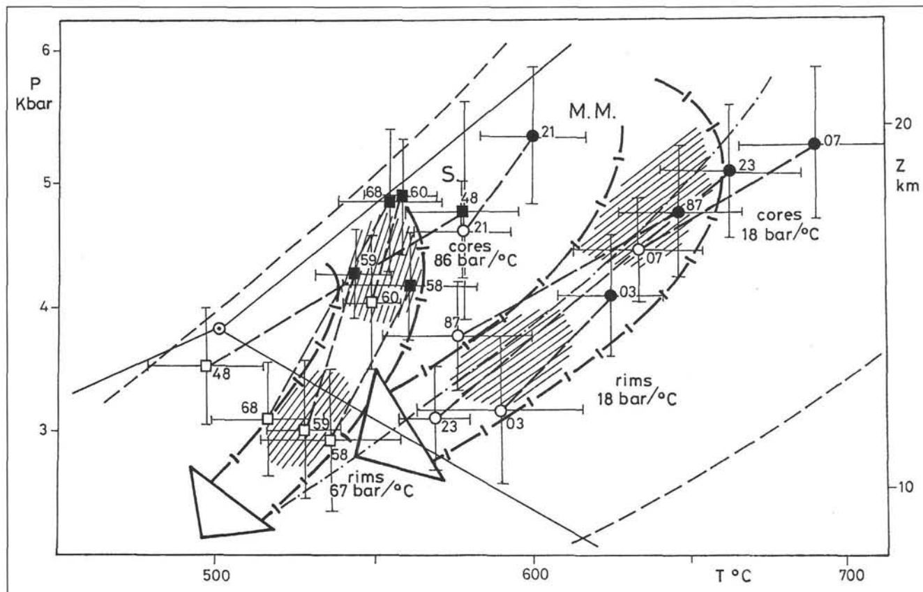
Text-Fig. 7. Generalized P–T conditions of metamorphism of Suchy (S.) and Mala Magura (M.M.) Mts. paragneisses. Slopes of the metamorphic reactions ( dP/dT ) in the simplified metamorphic system KMFASH including mineral phases St, Grt, Bt, Ms, Sil, Qtz were used (DYDA, 1990) to approximate the uplift conditions. The methodical approach was taken over from SPEAR & SELVERSTONE (1983), and SPEAR (1988). Triple point Al_2SiO_5 is after HOLDAWAY (1971).
