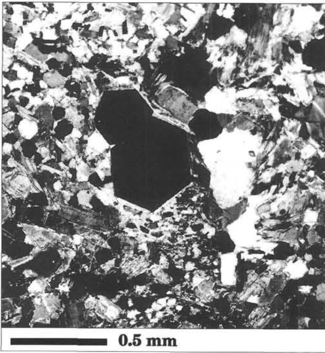
Text-Fig. 4. Idioblastic garnets with no resorption and decompression reaction signs demonstrate static periplutonic growth and are represented by the linear size distribution (population density versus crystal size). Sample M.K. 17. Cross-polarized light.
