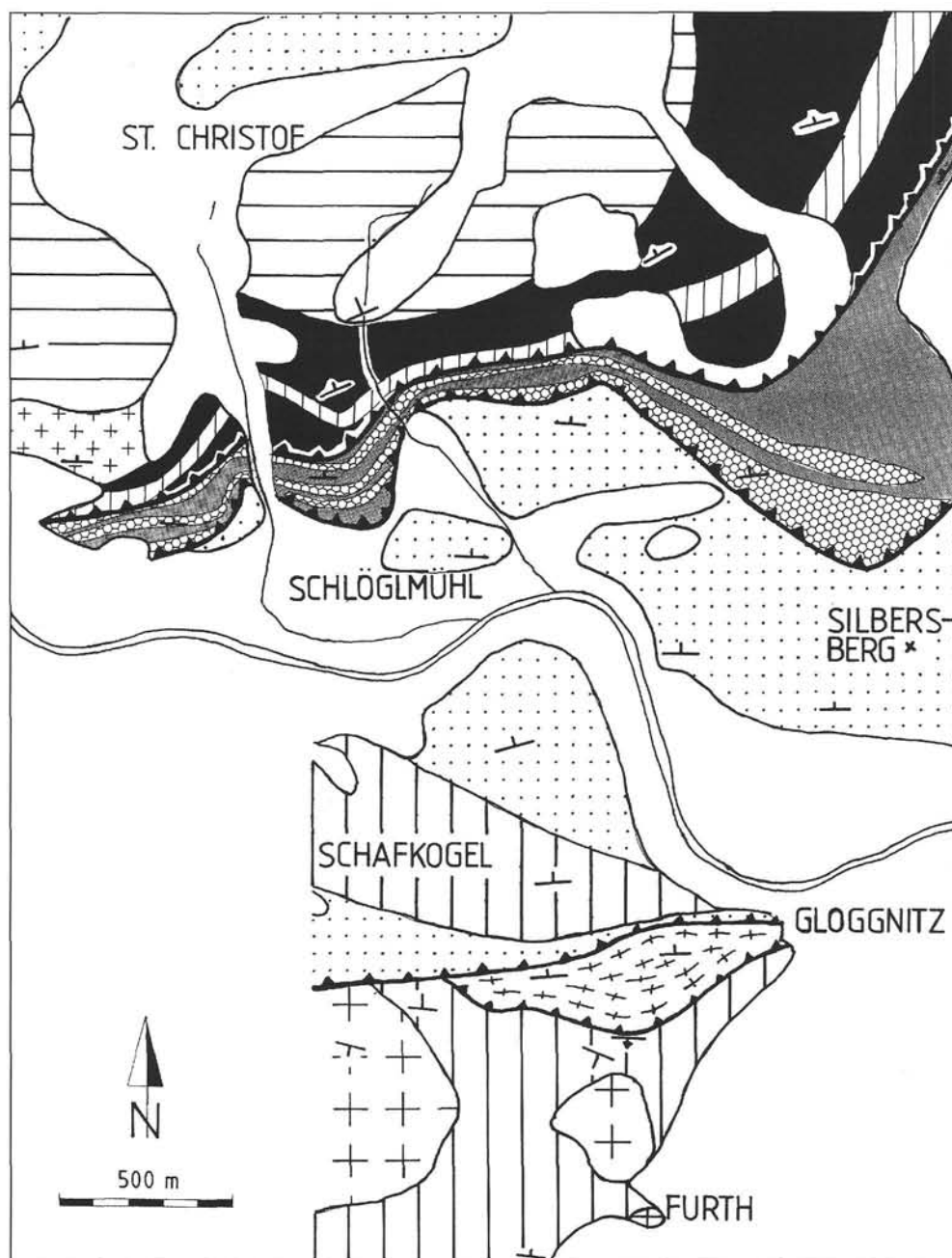
Text-Fig. 4. Simplified geological map of the Gloggnitz area. For location, see Text-Fig. 1; for legend, see Text-Fig. 3.
