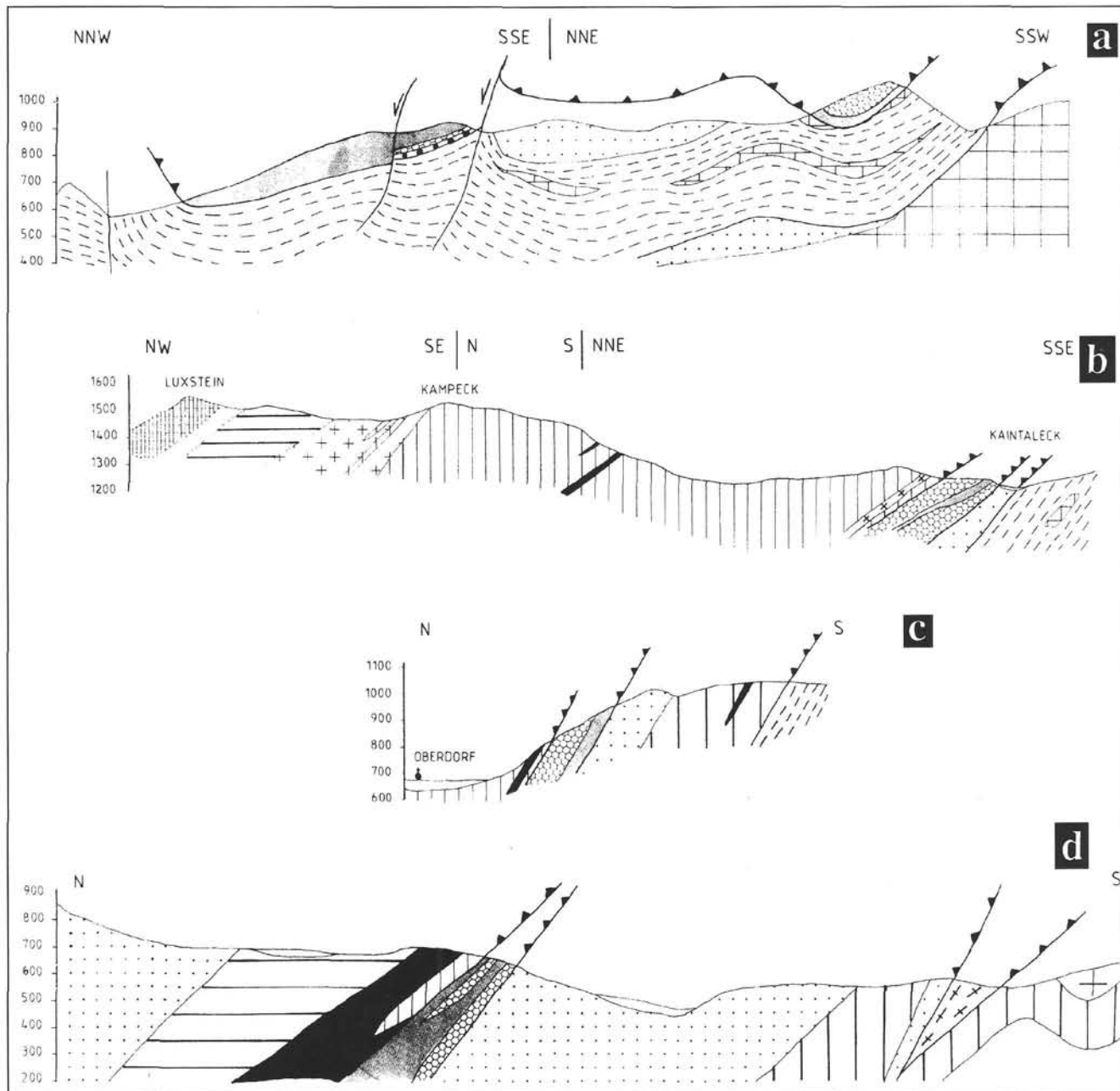
Text-Fig. 5. Sections of the eastern Graywacke Zone. For locations, see Text-Fig. 1. For legend, see Text-Fig. 3. Location of sections: a – Text-Fig. 2; b,c – Text-Fig. 3; d – Text-Fig. 4.
