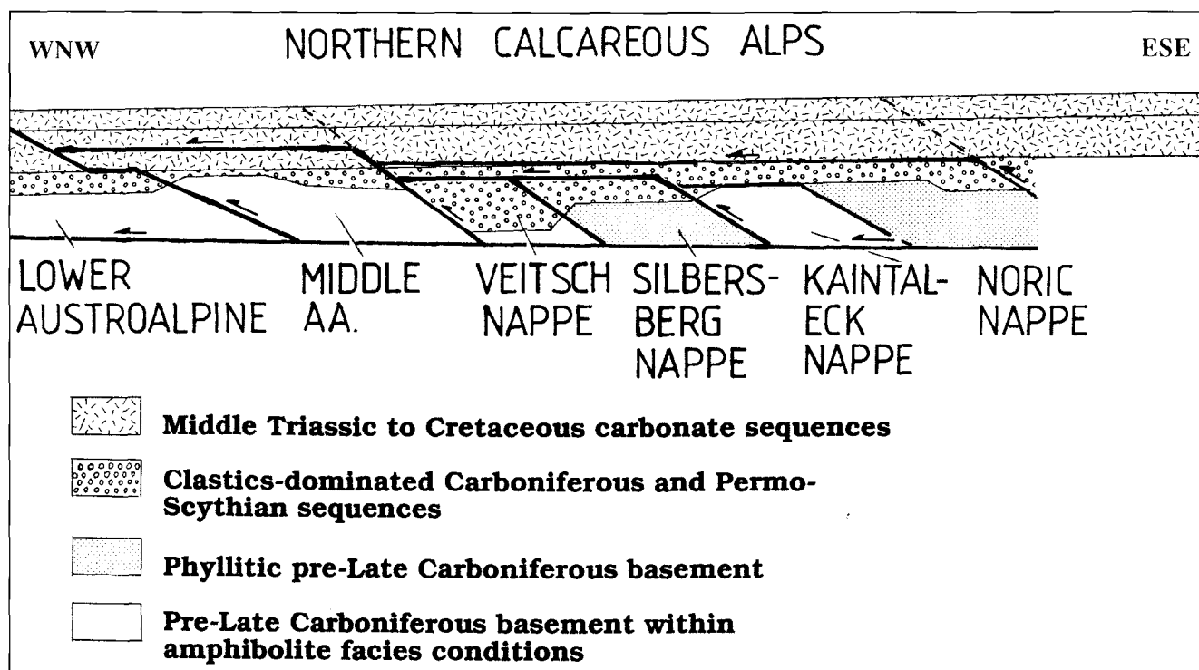
Text-Fig. 7. Suggested restored paleogeography of eastern sectors of the Austroalpine units.
