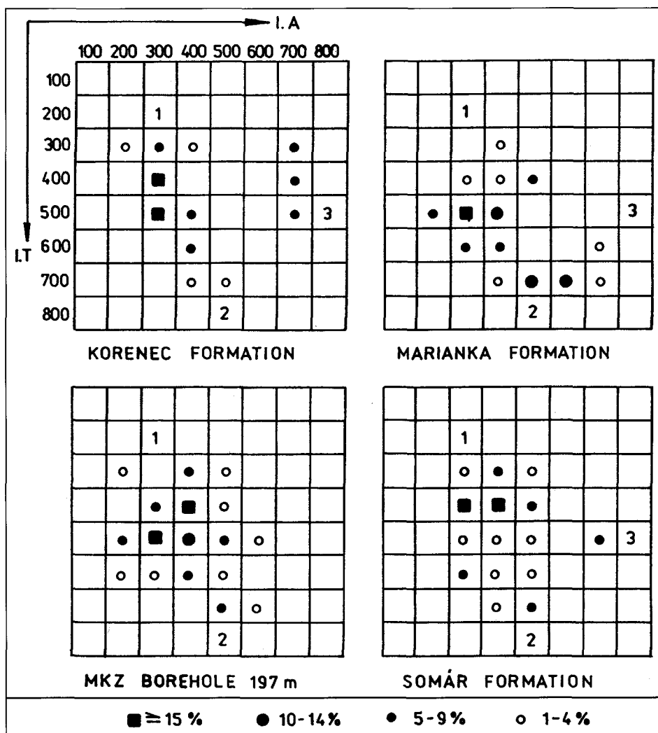
Text-Fig. 5. Percentages of zircon types from the Borinka unit. I.A = Appaicity index, I.T = Temperature index sensu PUPIN & TURCO, 1972; numbers in the diagram sign the three distinguished source-rocks.
