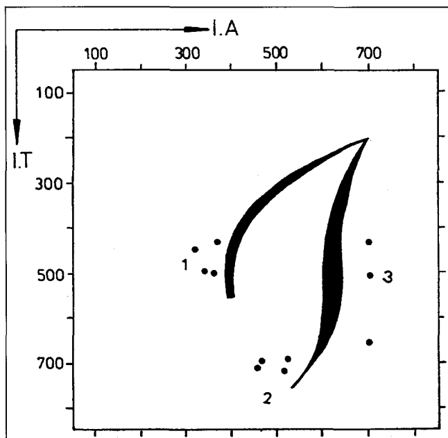
Text-Fig. 6. The mean values of the sources of clastic zircon from the Borinka unit. The thick line separates the fields of the rocks of crustal origin (left), hybrid rocks (middle) and rocks of mantle origin (right).
