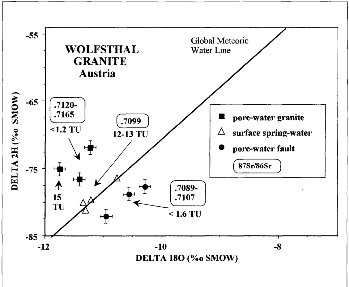
Fig. 13 Delta ^2\text{H} - ^{18}\text{O} - plot for pore- waters of granite and fault-gouges obtained by vacuum- extraction and ^{87}\text{Sr}/^{86}\text{Sr} ratios of leachates. Bars repre- sent standard error. Notice that the granite pore- water containing tritium (15 TU) is closest ( <50\text{ m} ) to the gallery entrance.
