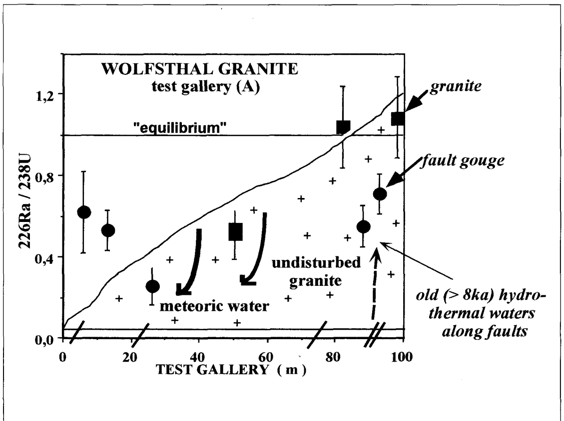
Fig. 14 ^{226}\text{Ra}/^{238}\text{U} ratio for fault- gouges and granites vs. test-gallery meter and interpretation of meteoric water seepage based on ^3\text{H} , \text{D} , ^{18}\text{O} , ^{87}\text{Sr} isotope measure- ments. Filled dots: Fault gouges left and right of the gallery. Filled squares: granite samples. The bars repre- sent standard error.
