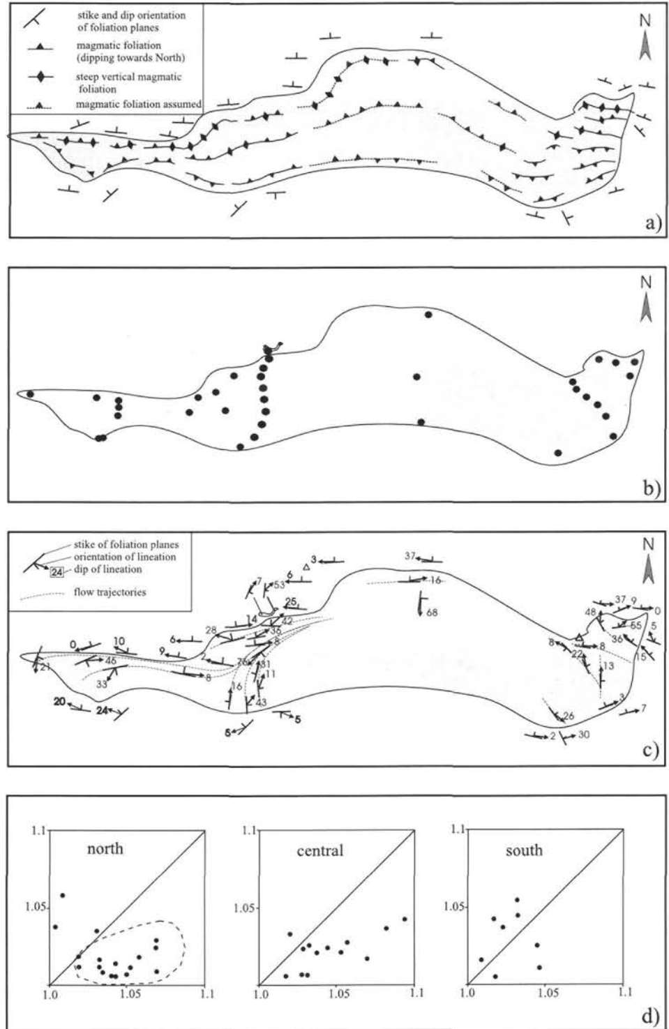
Fig. 11 a) Magmatic foliation planes from field observations and foliation planes of country rocks. Because of the intense erosion of the granitoid massif, the style of foliation is assumed along the Vals Valley. b) Sample points for AMS measurements within the Rensen massif. c) AMS data, only from samples with magmatic and sub-magmatic textures, indicate strike and dip of magnetic foliation and lineation within the pluton. Amount of magnetic lineation dip is indicated. Field measurements of cleavage in country rocks are shown outside the pluton. The magnetic lineation and foliation is predominantly E-W oriented north of the pluton. Central and southern areas indicate no directly preferred orientation of magnetic lineation and foliation. d) Flinn plots show prolate and oblate geometries within different sectors of the massif. Samples of the northern area (tonalitic rim) plot mostly within the oblate section whereas samples of central and southern parts show variable patterns trending to prolate geometries.
