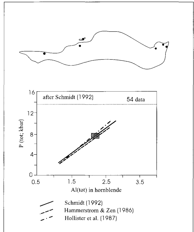
Fig. 13 Estimate of pressure during crystallisation of tonalite within the Rensen intrusion using Al tot in hornblende. Box indicates range of pressure using different calibrations and range of hornblende analyses. Shape of the Rensen shows locations of sample points for barometric estimates.
