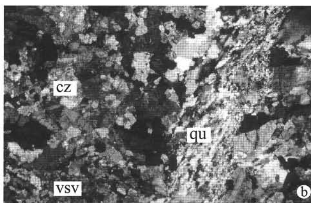
Fig. 15 a) Scarn mineral assemblage defined by the equilibrium of wollastonite (wo), phlogopite (phl) and clinozoisite (cz). Calcite (cc) occurs at the upper rim of the section. b) Recrystallized quartz (qu) within the scarn assemblage indicates syn-deformative fluid flow during cooling of magma. vsv (vesuvianite), cz (clinozoisite). Width of views: 3 mm.
