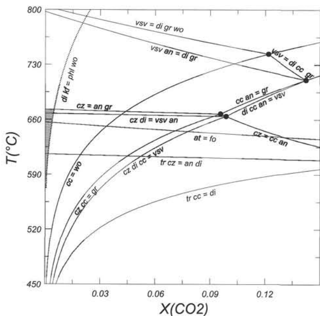
Fig. 14 Temperature estimate for the contact aureole based on scarn mineral assemblages. The diagram includes the constructed univariant mineral reaction lines and invariant points of the \text{SiO}_2 saturated system combined with a univariant reaction line ( \text{di kf} = \text{phl wo} ) of the \text{CaO} saturated system (dotted line). It is constructed by using the software Perplex (after CONNOLLY, 1990). Calculations are performed for 7.5 kbar, based on hornblende barometry; X_{\text{CO}_2} ranges between 0 and 0.15. Information for the temperature results by the occurrence of phlogopite and clinozoisite (shaded field), which occur together in equilibrium. Reaction equations are written by considering high temperature assemblages on the right of the "=" sign. Abbreviation of minerals is defined in the text.
