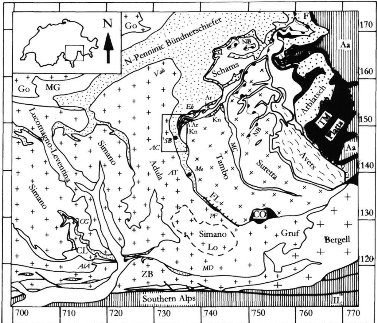
Fig. 2. Tectonic overview of the eastern Lepontine area. Aa: Austroalpine units; Ar: Areua slice; CL: Cima Lunga unit; CO: Chiavenna ophiolite; F: Flysch; FL: Forcola Line, Go: Gotthard "massif"; IL: Insubric Line; Kn: Knorren mélangé; Lo: Lostalio window; MC: Mesozoic cover of the Suretta and Tambo nappes; MG: Mesozoic cover of the Gotthard "massif"; NB: Axial trace of the Niemet-Beverin fold; TM: Turba mylonite zone; ZB: Bellinzona-Dascio zone. AC: Alp de Confin; AIA: Alpe Arami; AT: Alp de Trescolmen; CG: Cima di Gagnone; Eh: Einshorn; MD: Monte Duria; Me: Mesocco; PF: Passo della Forcola; SB: San Bernardino. Rectangle: Study area.
