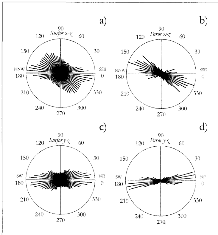
Fig.11 Rose diagrammes of orientation distributions (PANOZZO 1983, 1984) of recrystallized grain boundaries (SURFOR) and grain long axes (PAROR) in sample A48 (see Fig. 10). a) SURFOR analysis of the x-z section; b) PAROR analysis of the x-z section; c) SURFOR analysis of the y-z section; d) PAROR analysis of the y-z section.
