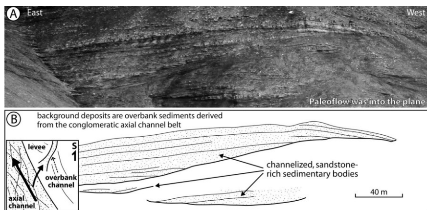
FIGURE 11: a) Overbank channel deposits in the Cerro Toro Formation. b) Annotated line-drawing trace of features in part (a). Inset map shows the relationship of overbank channels with the main axial channel (bold arrows indicate paleocurrent directions).
