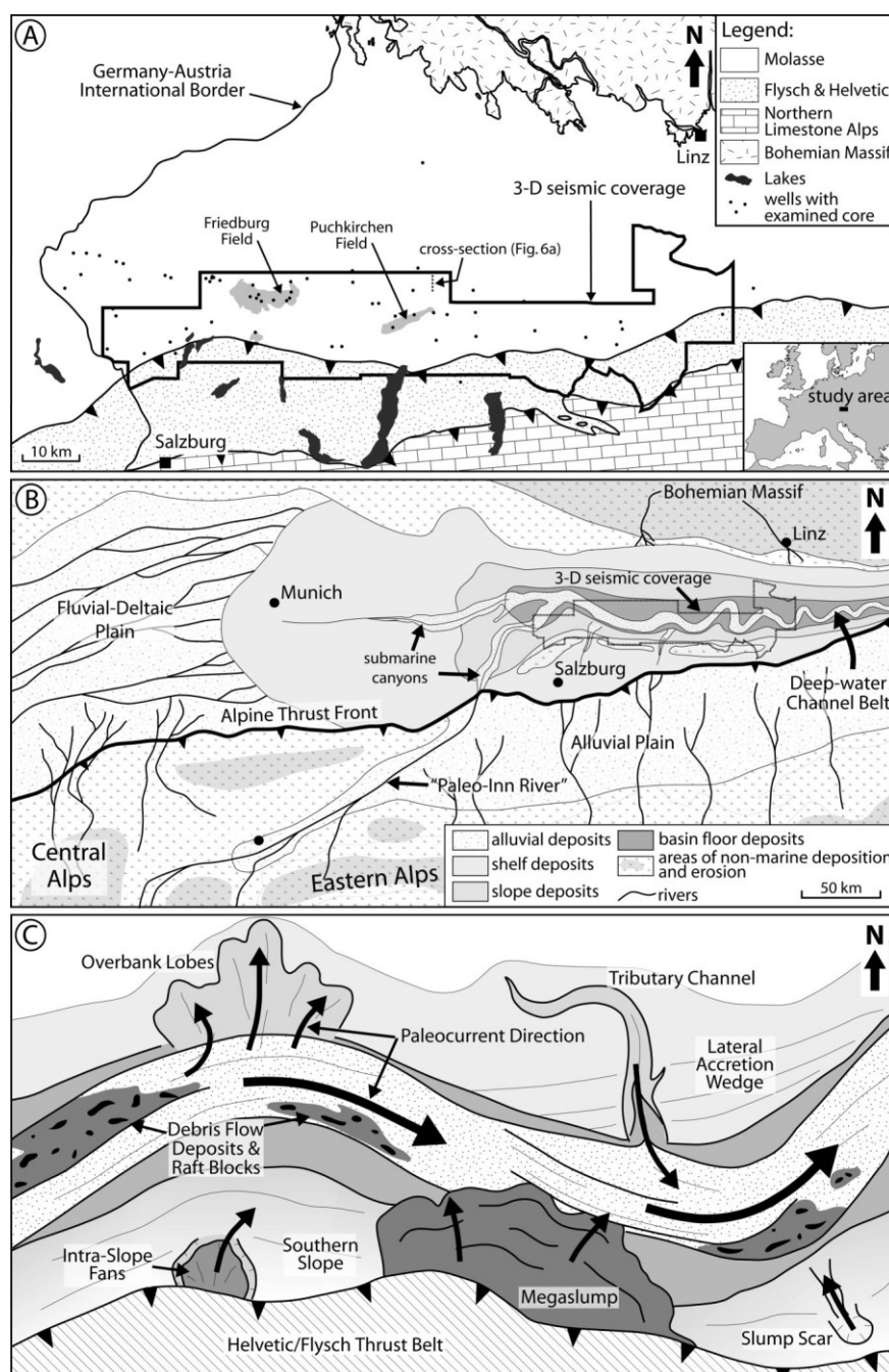
FIGURE 1: a) Upper Austria study area showing distribution of wells with deep-water cores analyzed, as well as the area covered by 3D seismic data. b) Interpreted Oligocene-Miocene paleogeography of the Central and Eastern Alps, and the Molasse Basin. Note the location of the extensive, east-west trending channel belt present along the Molasse Basin axis (modified from de Ruig and Hubbard (in press), with data from Frisch et al. (1998) and Ortnér and Stingl (2001)). c) Interpreted depositional model for deep-water channel deposition in the Molasse Basin (modified from de Ruig and Hubbard, in press). The channel belt ranges in width from 3 to 5 km.
