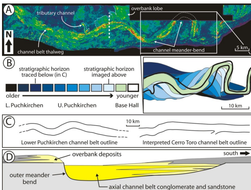
FIGURE 5: a) 3D seismic image highlighting channel features through ~40 m of strata in the upper part of the Puchkirchen Formation. Bright areas correspond to conglomeratic deposits in the channel thalweg, whereas darker areas are associated with finer out-of-channel deposits (overbank, slope). Images like this were made for eleven successive stratigraphic layers, from the upper part of the Lower Puchkirchen Formation into the overlying Basal Hall Formation. The outline of the channel belt thalweg from each interval, stacked on top of one another is present in part (b) (modified from de Ruig and Hubbard, in press). Note the shifts in channel meander loops from west to east, indicating that paleoflow was eastward during deposition of the formation. c) Outline of basin axial channel belts in the Lower Puchkirchen and Cerro Toro formations showing the similarity in scale of the two systems. The outline of the channel in the Cerro Toro Formation is based on mapping of field exposures of coarse-grained deposits in the Chilean outcrop belt (from Hubbard et al., in press a). d) Schematic cross-sectional model for channel deposition in the Puchkirchen Formation (modified from de Ruig, 2003). Paleoflow direction was into the plane. The channel belt is asymmetric, associated with significant erosion on the outer edge of meander bends and lesser erosion and more aggradation on the inner edge of meander bends. See vertical dashed line in part (a) for approximate location (channel is 3-5 km wide).
