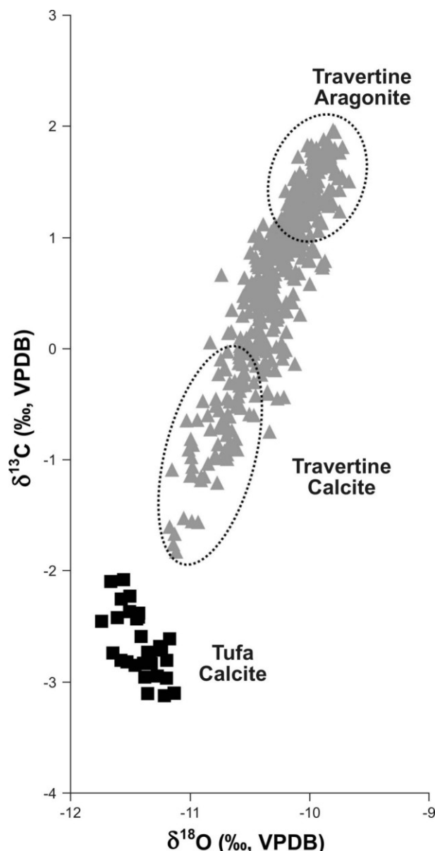
FIGURE 5: Stable isotopic analyses of travertine and tufa samples from Ainert. The two circles define the compositions of aragonite and calcite endmembers. For details see text.
