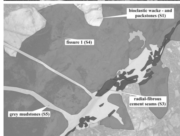
FIGURE 6: Detail of fissure 1 showing four different ages of sedimentation (S1, S3–S5).
