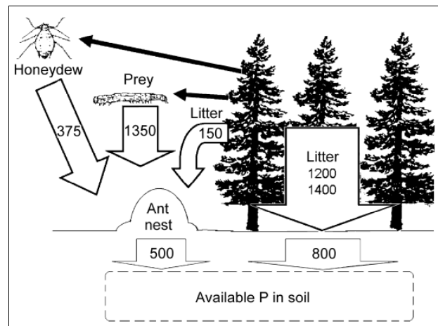
Fig. 2: The effect of the wood ant Formica polyctena on P availability (g of P per ha per year) in a forest ecosystem. The upper parts of the scheme represent the flow of total P. The bottom parts summarize the annual input of available P in individual compartments. Based on data from FROUZ & al. (1997).
