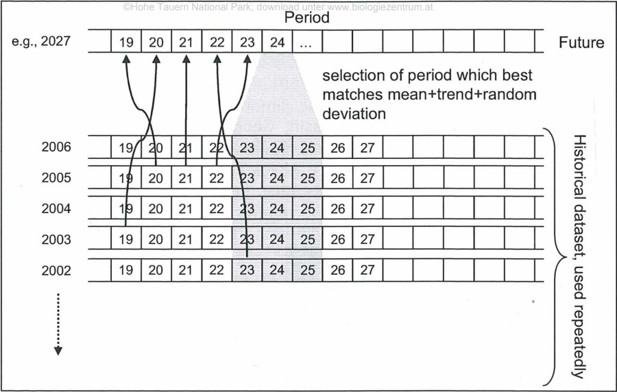
Figure 2: Principle of selecting periods of measured data to build up a future data time series with a certain temperature trend and random deviation.
