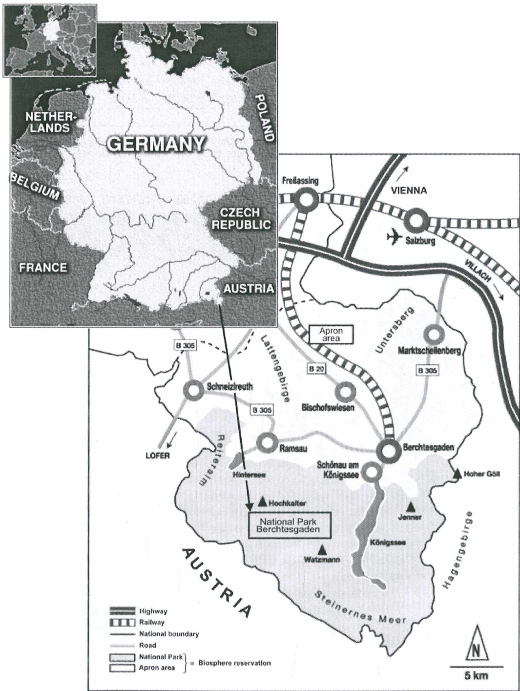
Figure 1: Location of the Berchtesgaden National Park (Germany).
