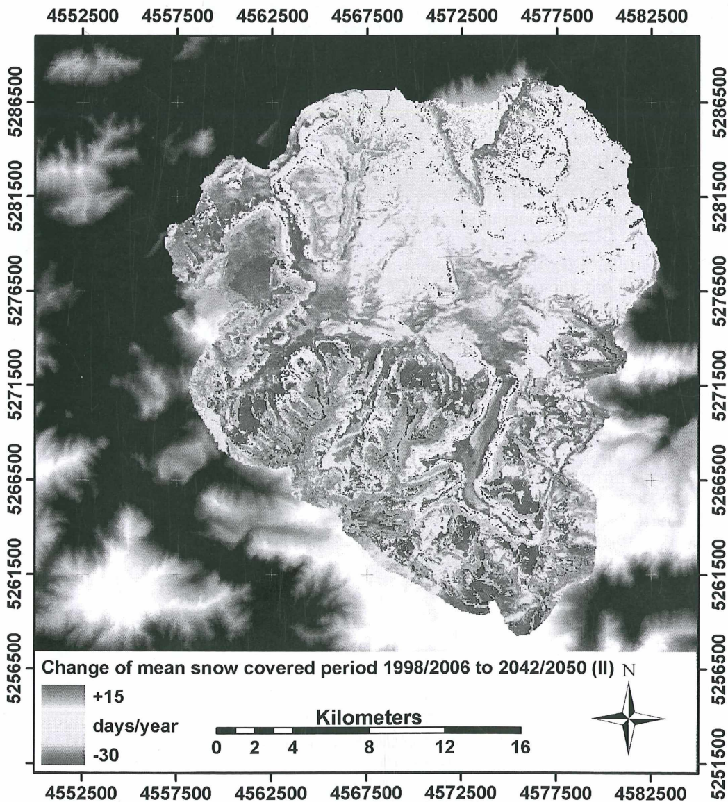
Figure 3: Mean annual difference in the duration of the snow-covered period between 2042–2050 under scenario conditions and the reference period 1998–2006.
