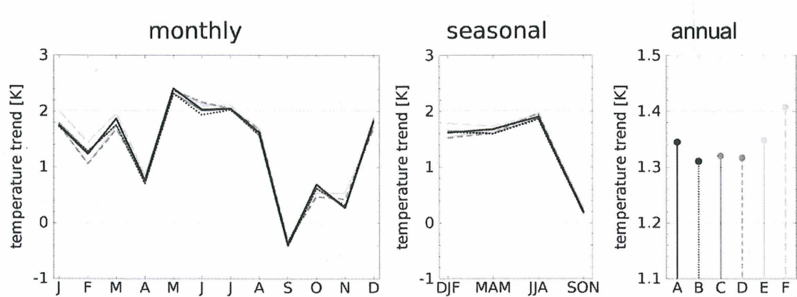
Figure 3: Monthly, seasonal and annual absolute temperature trends at the six selected sites in 2500m a.s.l. 1961-2006: A=Pasterze Glacier (black line), B=Schareck - Fallbichl (black dots), C=Central Schober Mountains (grey line), D=Dösen Valley (grey broken), E=Hintereggen Valley (light grey) and F=Hochreichart (light grey broken).
