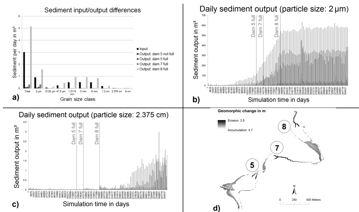
Figure 4: Modelling results for the dam construction scenario (examples): sediment outputs for a) all grain size classes, b) suspended sediments, c) bedload sediments; d) geomorphic channel changes
