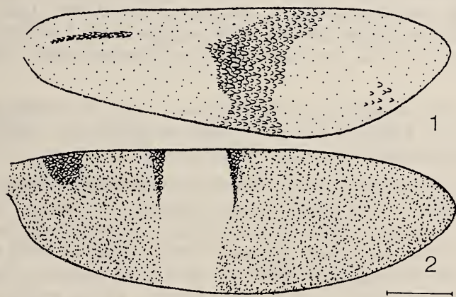
Figs. 1-2. Forewing pattern: 1 — Nemophora sinevi sp. n.; 2 — N. ochrocephala sp. n. (reference bar 1 mm).
