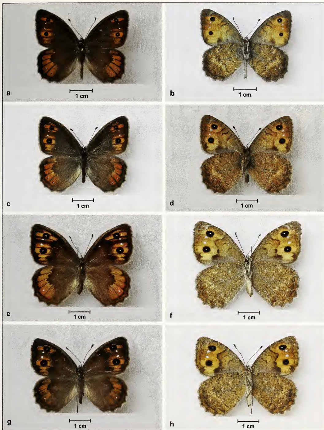
Figure 5. Variability in P. mniszecii tisiphone . a–b. Typical ♂ upper- and underside, Boboshtiçë, Albania, 16.vii.2013. c–d. ♂ typical upper- and underside, Boboshtiçë, Albania, 16.vii.2013. e–f. ♀ typical upper- and underside, Boboshtiçë, Albania, 16.vii.2013. g–h. ♀ dark form upper- and underside, Boboshtiçë, Albania, 18.vii.2013. (Coll. & photographs: SC).
