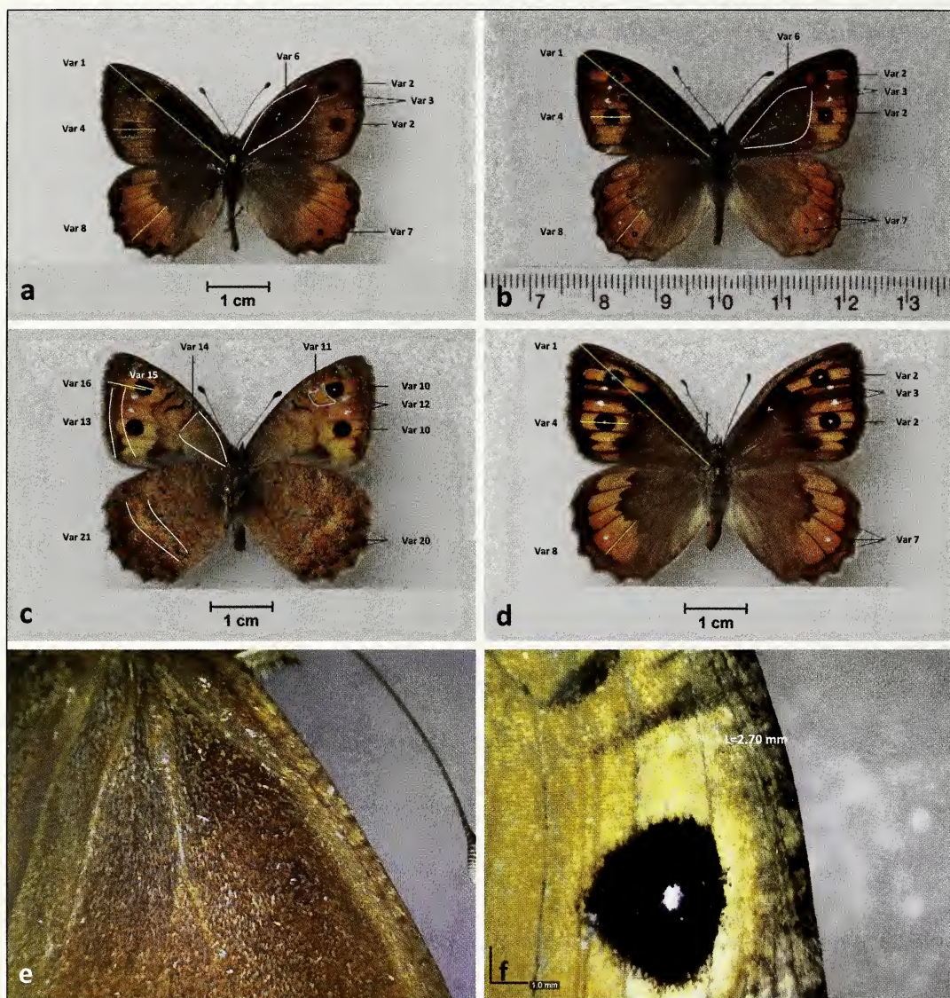
Variables of P. amymone and P. mnischezii tisiphone . a. UPS variables of ♂ P. amymone , Boboshtiçë, Albania, 16.vii.2013. b. UPS variables of ♂ P. mnischezii tisiphone , Boboshtiçë, Albania, 16.vii.2013. c. UNS variables of ♂ P. mnischezii tisiphone , Boboshtiçë, Albania, 16.vii.2013. d. UPS variables of ♀ P. mnischezii tisiphone , Boboshtiçë, Albania, 16.vii.2013. e. Sex brand of ♂ P. amymone (×30), Boboshtiçë, Albania, 16.vii.2013. f. UNS pale area from ocellus in S5 towards cell, P. amymone (×32), Boboshtiçë, Albania, 16.vii.2013. (Coll. & photographs: SC).
