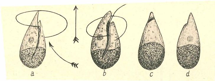
Entomosigma peridinioides , sp. nov. — 1600 \times vergr.
