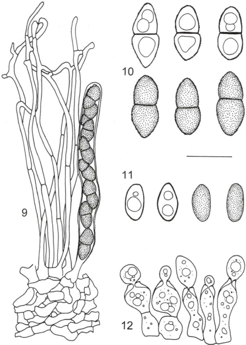
Figs. 9-12. Line drawings of selected features of Immotthia atrograna . Fig. 9. Part of hymenium showing hamathecium and asci. Fig. 10. Ascospores. Fig. 11. Presumed anamorph: conidia. Fig. 12. Presumed anamorph: conidiogenous cells. Bars: Fig. 9: 20 \mu m, Figs. 10-12: 10 \mu m.
