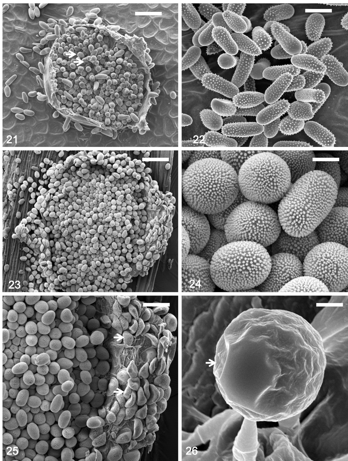
Figs. 21–26. Surface structures of sori and spores of Melampsora laricis-populina observed under SEM. – Fig. 21. An uredinium on Populus x canadensis . Urediniospores and abundant paraphyses (allow) are observed in an uredinium. Scale bar 40 \mu\text{m} . – Fig. 22. Urediniospores. Their surfaces are echinulate except smooth apex parts. Scale bar 20 \mu\text{m} . – Fig. 23. Caeoma -type aecium on Larix olgensis . Scale bar 100 \mu\text{m} . – Fig. 24. Verrucose aeciospores. Scale bar 10 \mu\text{m} . – Fig. 25. Rudimentary peridia in an aecium (allow). Scale bar 50 \mu\text{m} . – Fig. 26. A basidiospore. Minute projection (allow) on the surface. Scale bar 2 \mu\text{m} .
