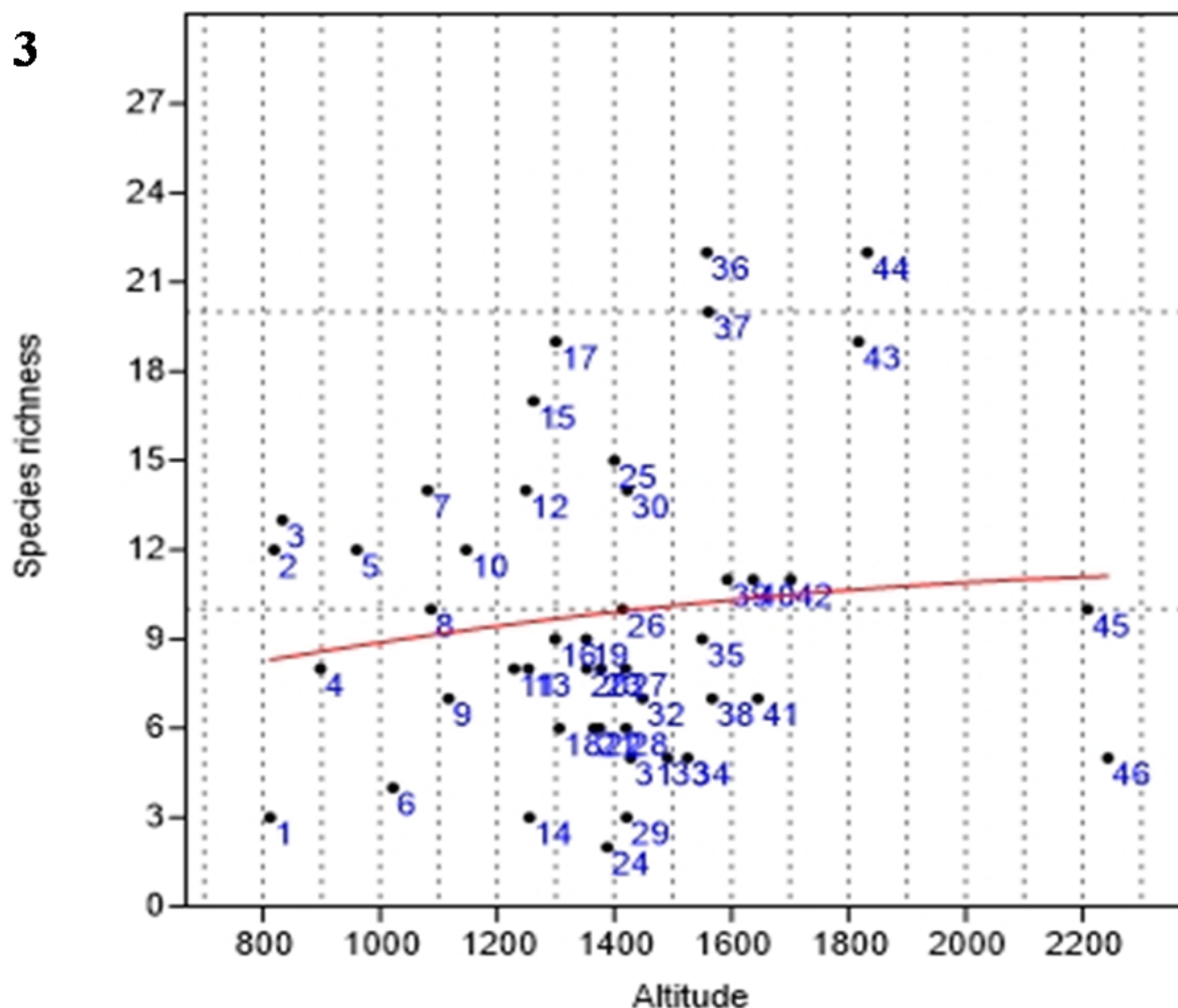
Fig. 3. Polynomial regression analysis between altitude and species richness of lichens ( Y = -9.096-07x^2 + 0.0047x + 5.052 , r^2 = 0.016 , p = 0.70 ).
