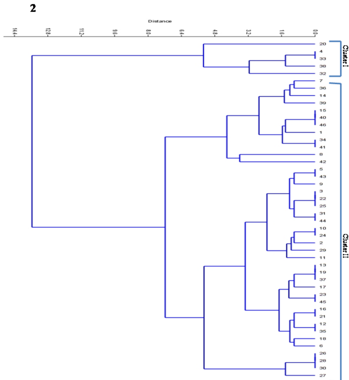
Fig. 2. Hierarchal cluster analysis between species richness of lichens on all the monuments and number of lichen families for the determination of compositional difference between monuments.
