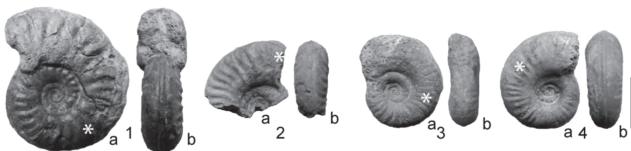
Fig. 3. Ammonites of the Gosheim Formation, 'Humphriesioolith' Member, Lower Bajocian, Humphriesianum Zone, Pinguis Subzone, ?deltafalcata biohorizon, Gosheim, road near ski lift [leg. N. WANNENMACHER †]. (1) Pelokodites sulcatum (BUCKMAN, 1893), a: lateral view, b: ventral view, SMNS 70635/1. (2) " Dorsetensia " sp., a: lateral view, b: ventral view, SMNS 70635/2. (3, 4) " Dorsetensia " punctatissima (HAUG, 1893), (3a, b) SMNS 70635/3 (4a, b) SMNS 70635/4. Scale bar equals 1 cm. All ammonites in natural size. Beginning of the body chamber is indicated by an asterisk.
