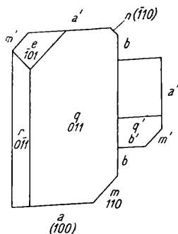
3, 4, 5-Tribromphenol.
