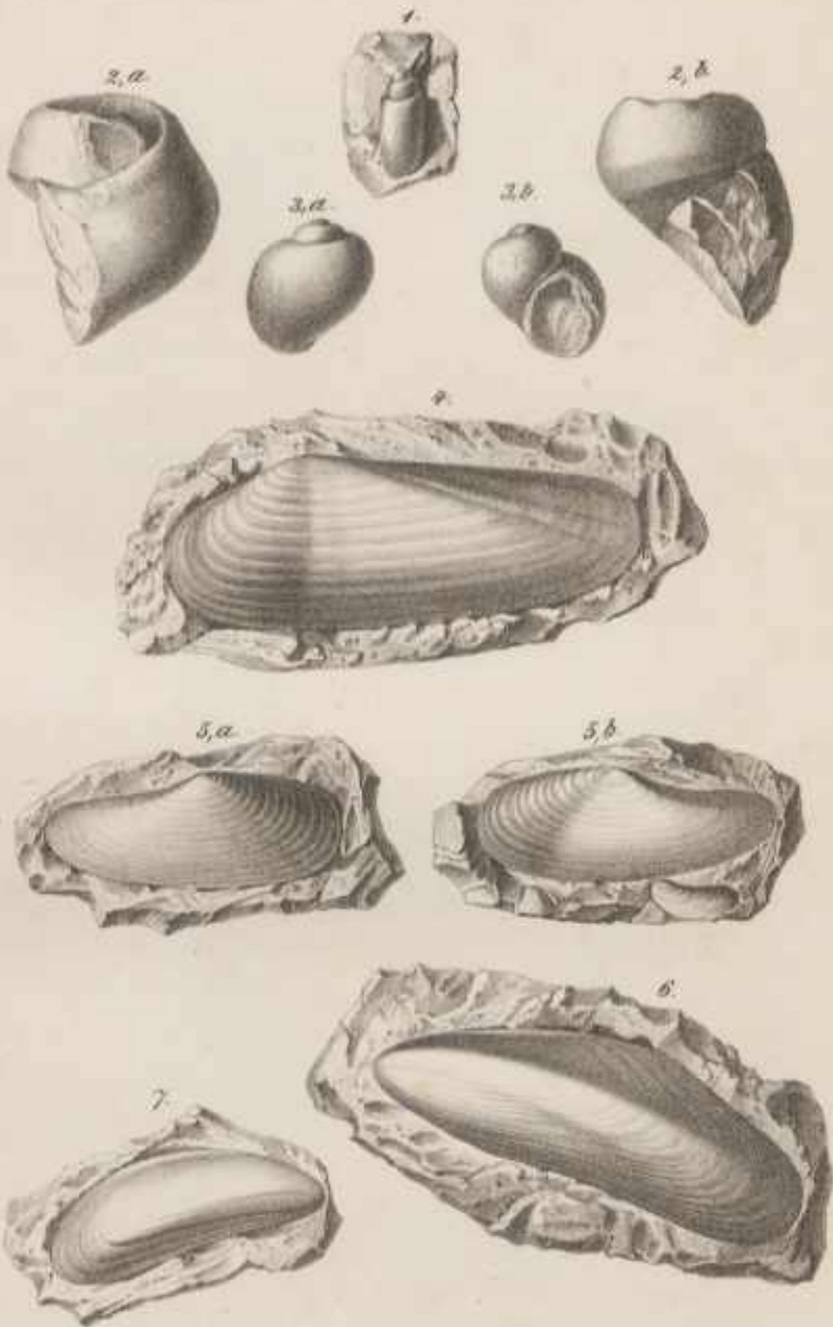
Fig. 1. Acteonina sp.
