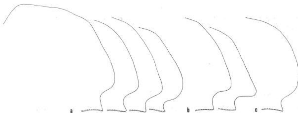
Fig. 24. Ctenophthalmus nifetodes ssp., outline of sternum VIII of males: a, b. C. n. petrovi ssp. n., (a) holotype and paratypes, (b) Komovi Mts., Montenegro; c. C. n. krystufeki ssp. n., holotype.
