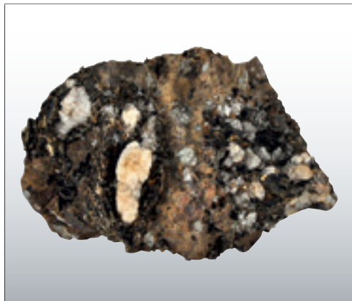
Glinenec, biotit in apatit v karbonatitu, Zizi, Selous Game Reserve
