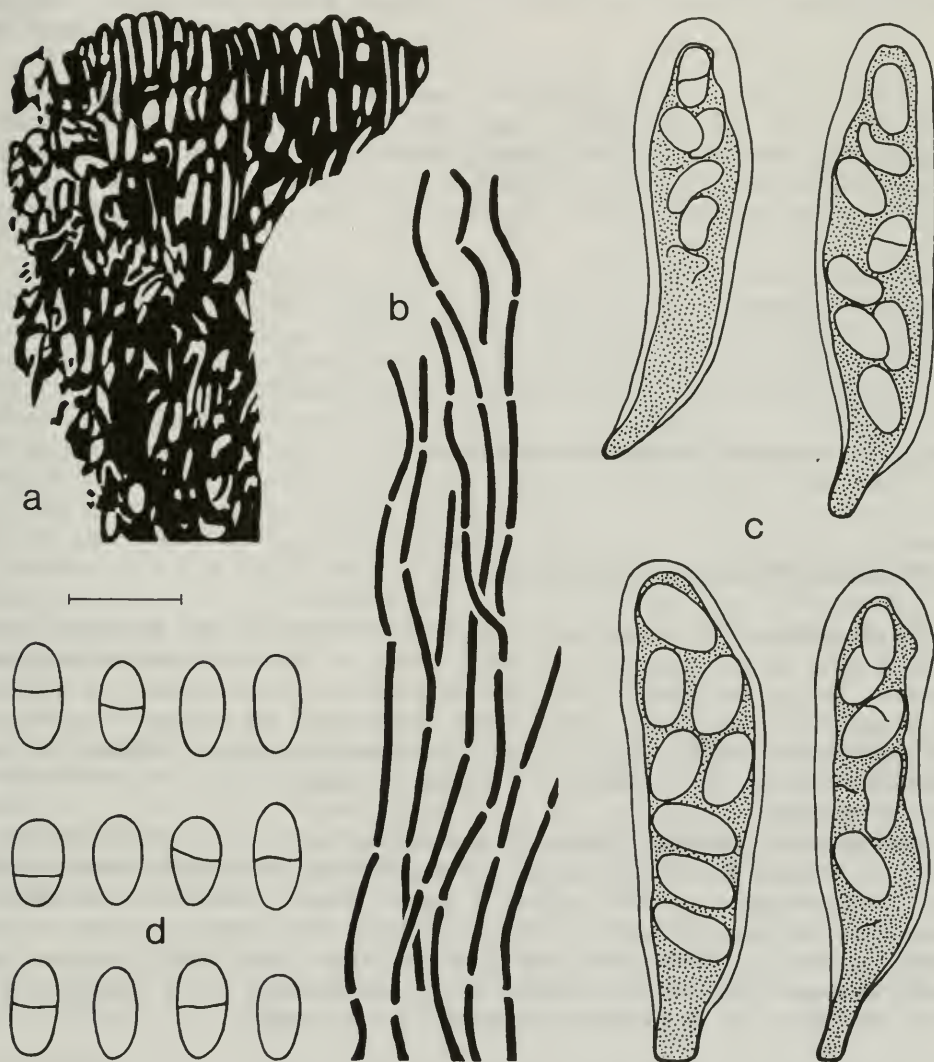
Fig. 1: Sagediopsis dissimilis : a) apical part of the ascomata wall; b) paraphysoids; c) asci; d) ascospores [a, c, d: in H_2O ; b: in lactophenol cotton blue; H. Hertel 29431 (M)]. – Scale: a: 18 \mu m ; b-d: 10 \mu m .
