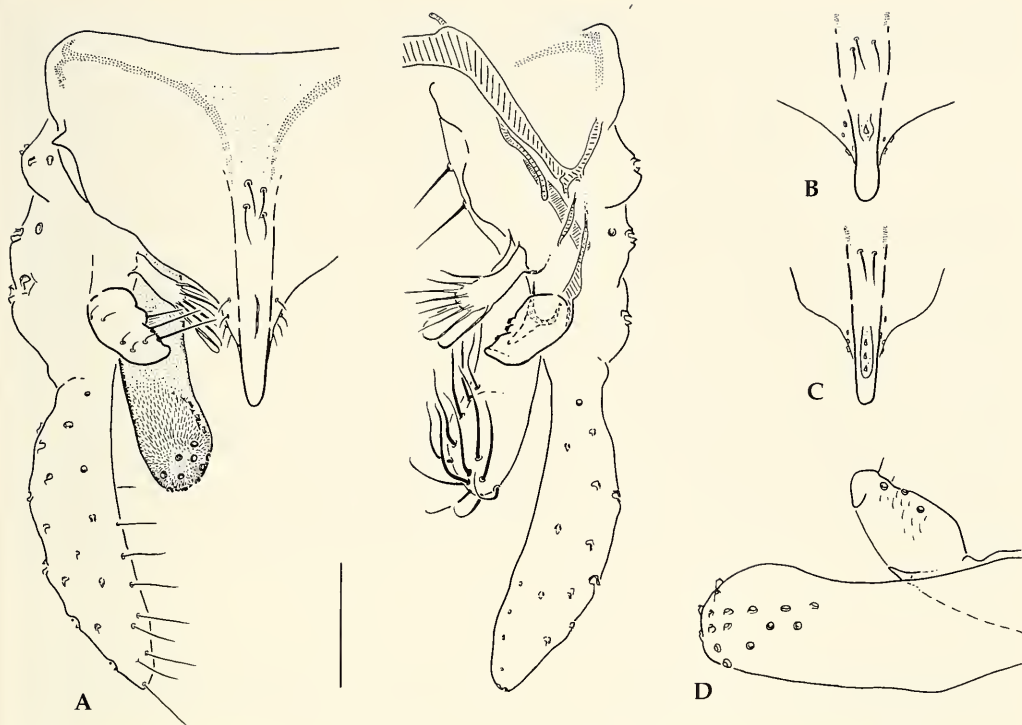
Fig. 2. Tanytarsus pelsuei , spec. nov. Adult male. A. Hypopygium, dorsal (scale 50 µm). B, C. Anal point variations, dorsal. D. Superior and inferior volsellae, median aspect.
