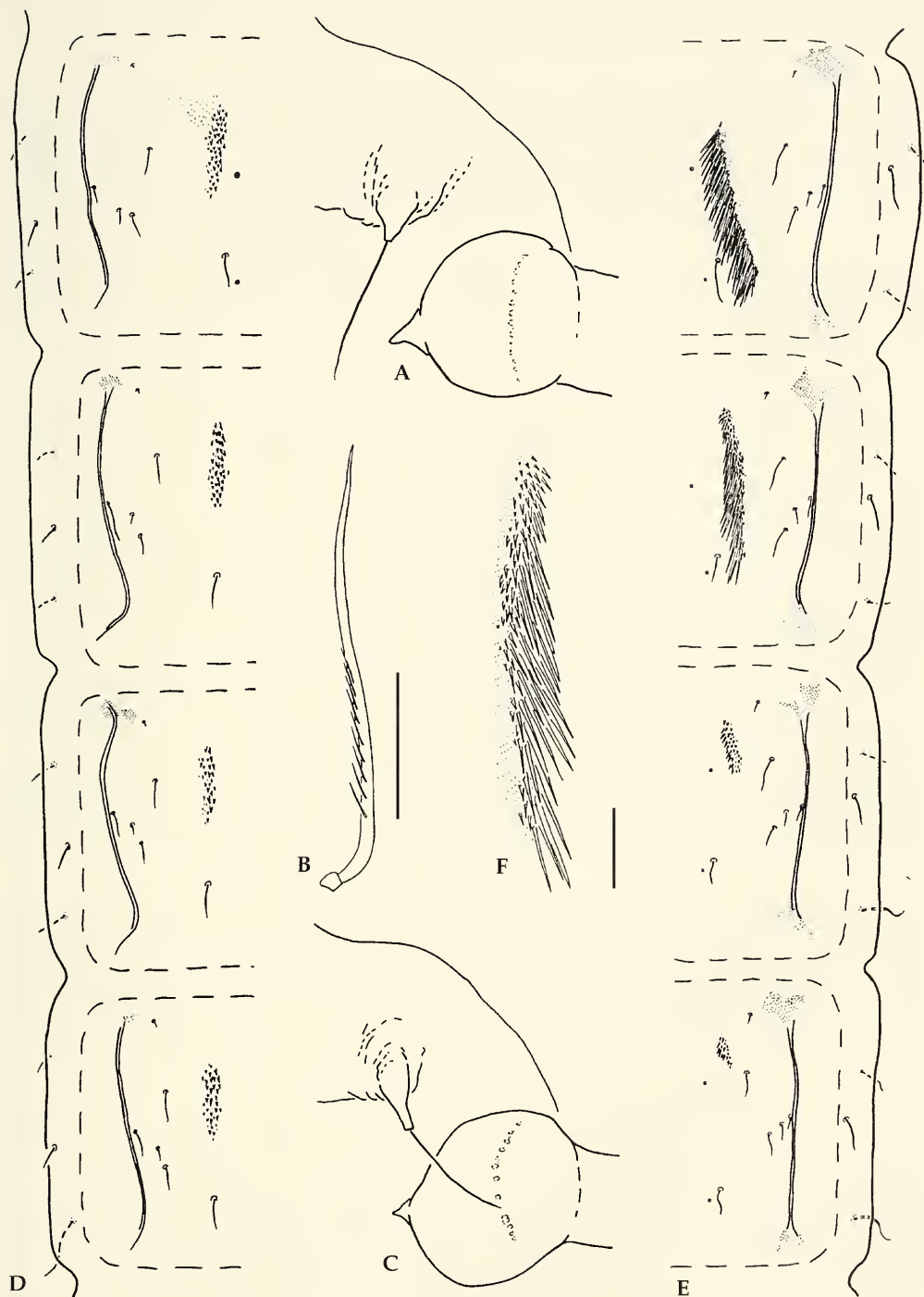
Fig. 5. Pupal structures of three species of Tanytarsus – A, C: frontal region; B: thoracic horn (scale 200 µm); D, E: abdominal terga III–VI; F: spine patch of TIV (scale 50 µm). A, B. T. challeti , spec. nov. C, D. T. pelsuei , spec. nov. E, F. T. angulatus Kawai.
