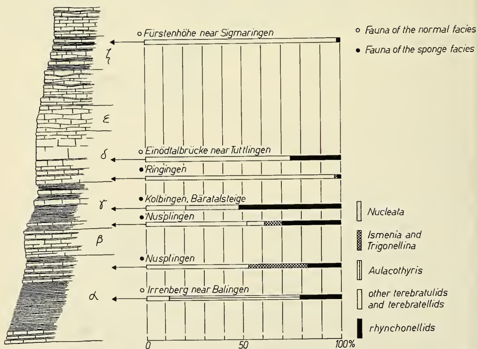
Fig. 33. Brachiopod faunas in the Swabian White Jurassic and their composition (according to individuals) of the most important groups.
