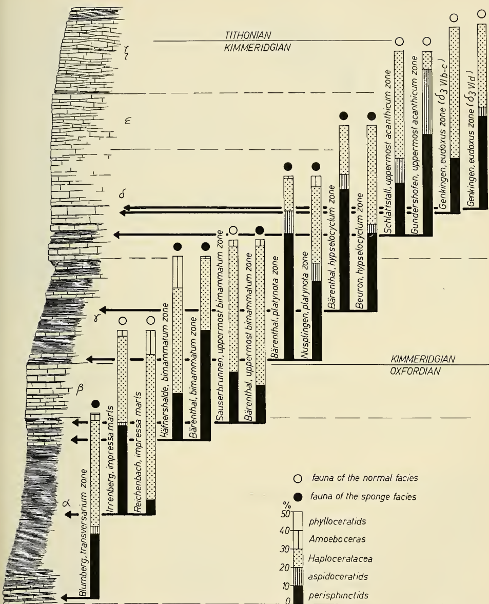
Fig. 34. Ammonite faunas in the Swabian White Jurassic and their composition (according to individuals) of the major ammonite groups.
