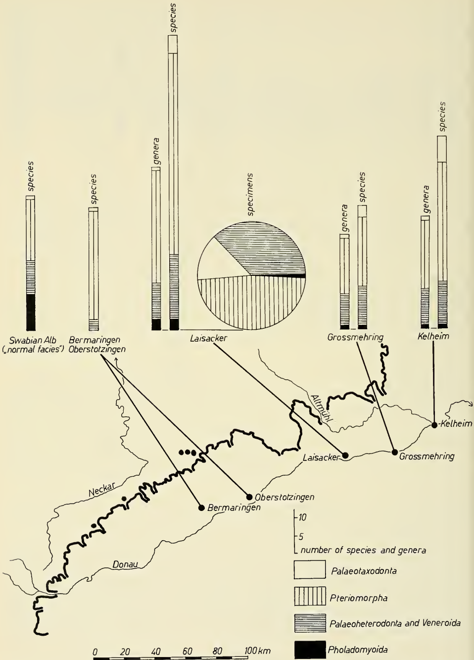
Fig. 42. The composition of major groups and the diversity of some pelecypod faunas of the upper Malm of southern Germany. Swabian Alb after TH. ENGEL (1908). Bermaringen and Oberstotzingen after O. F. GEYER (1953 a). Laisacker, Großmehring, and Kelheim after S.-A. YAMANI (1973; 1975; 1976), and S.-A. YAMANI & G. SCHAIRER (1975).
