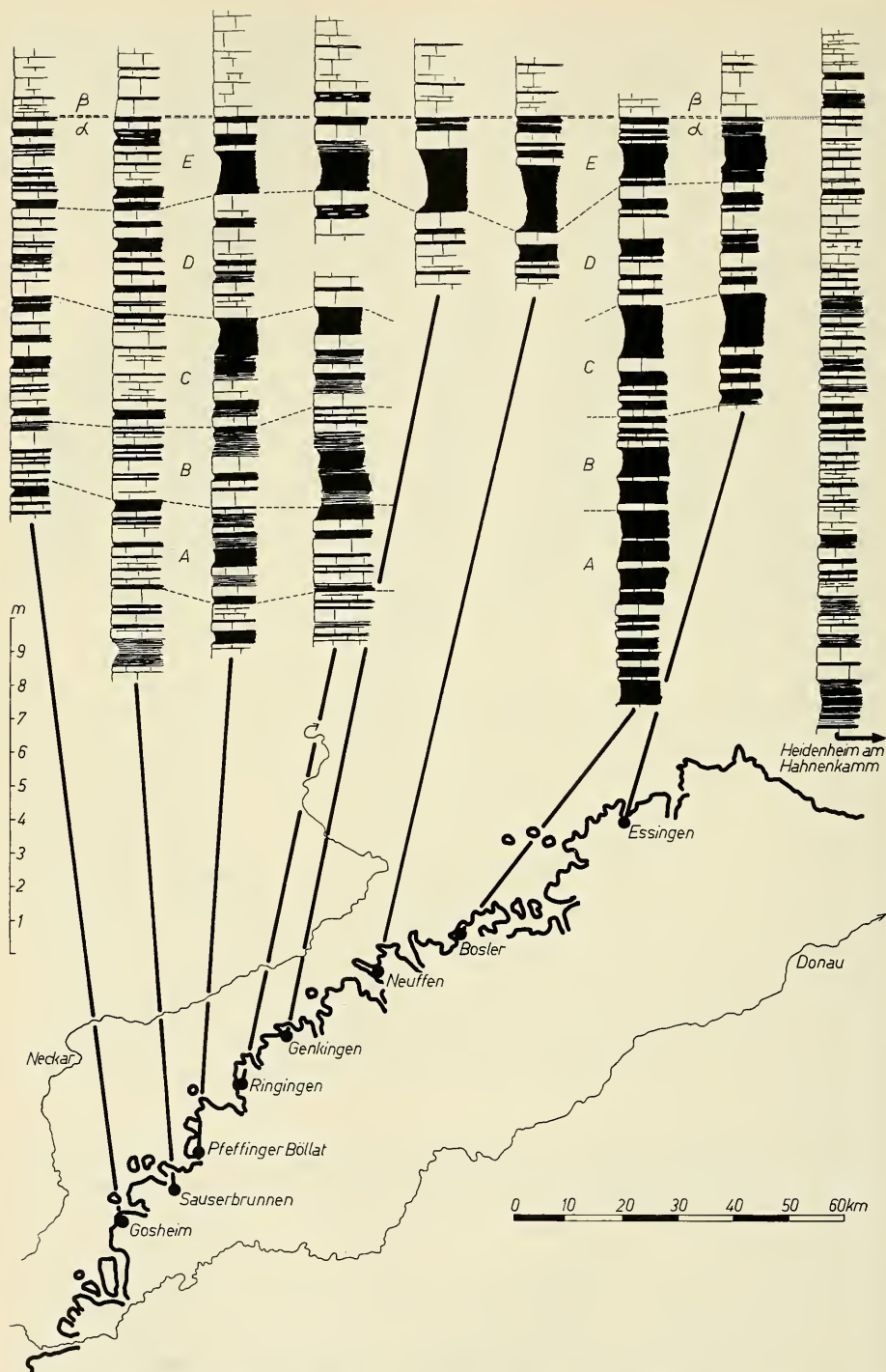
Fig. 4. The lithostratigraphy of the uppermost part of the White Jurassic \alpha . Sections Gosheim, Sauserbrunnen, Pfeffinger Böllat, Ringingen, and Genkingen after U. KOERNER (1963). Section Neuffen after E. & I. SEIBOLD (1953). Sections Bosler, Essingen, and Heidenheim am Hahnenkamm after H. SCHMIDT-KALER (1962 b).
