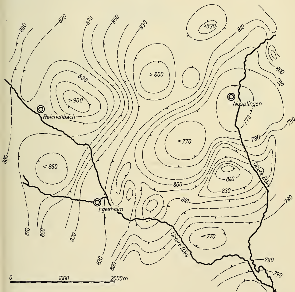
Fig. 27. The relief of the sponge-algal bioherms at the boundary between the White Jurassic \beta and \gamma (boundary Oxfordian/Kimmeridgian) near Nusplingen (southwestern Swabian Alb). Lines of equal elevation above sea level (in meters). After K. SCHÄDEL in B. ZIEGLER (1958 a).
