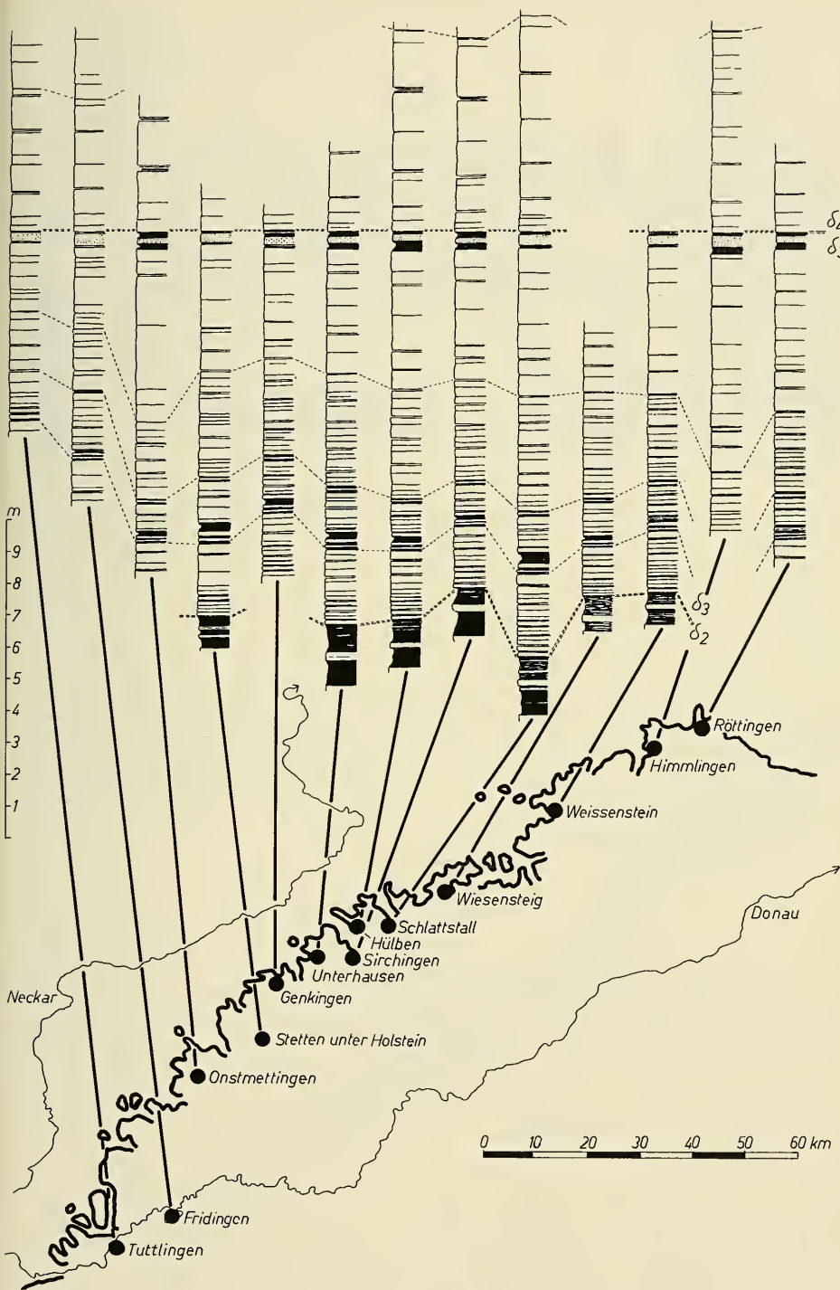
Fig. 9. The lithostratigraphy of the middle part of the White Jurassic \delta in the Swabian Alb. After B. ZIEGLER (1955; 1958 a; 1959).
