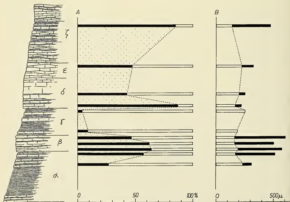
Fig. 22. The insoluble residues in some samples of the Swabian White Jurassic and the sizes of the grains. After G. KNOBLAUCH (1963).
