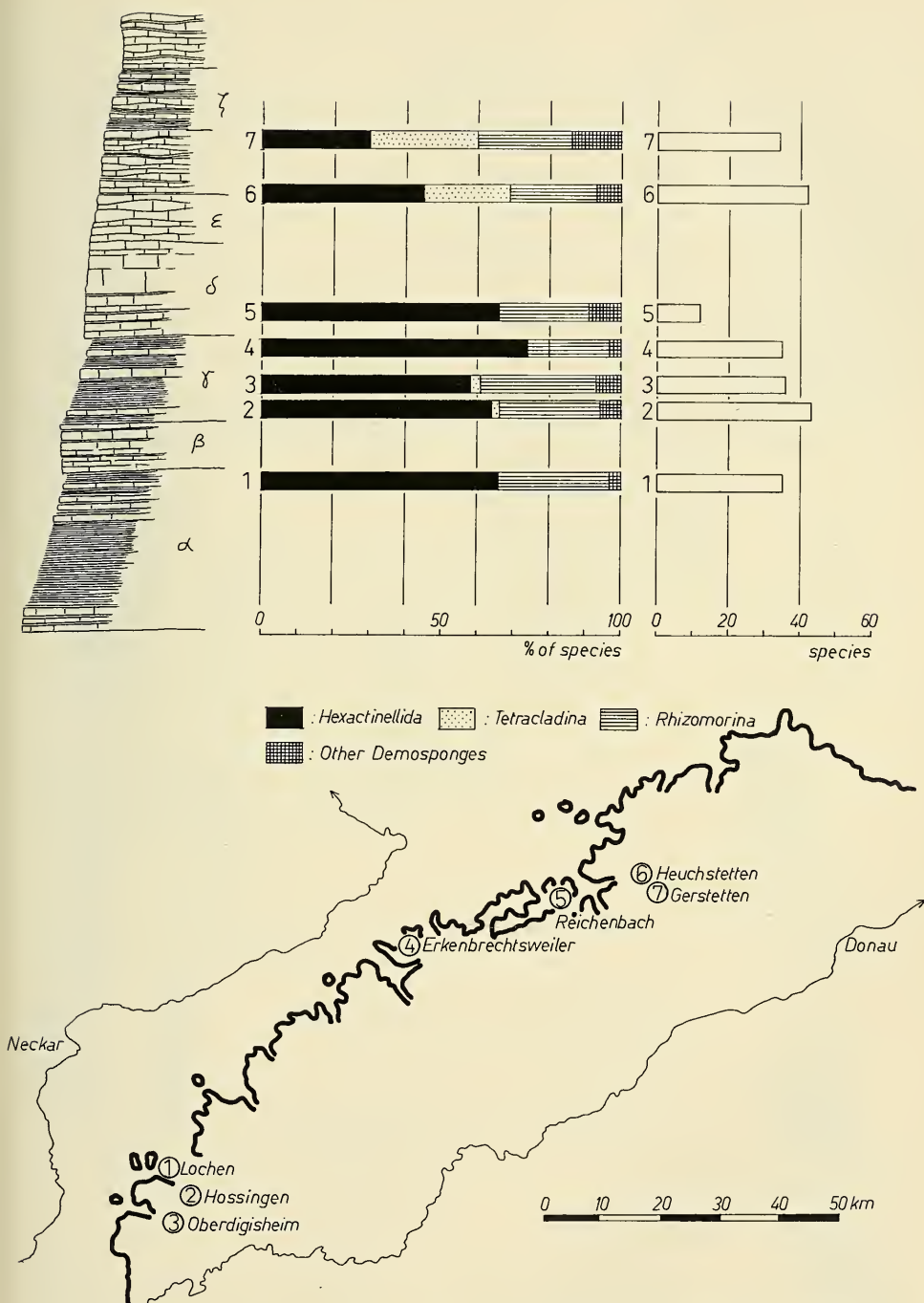
Fig. 31. Some characteristic faunas of siliceous sponges in the White Jurassic of the Swabian Alb. Note the reduction of Hexactinellida and the greater frequency of Tetracladina in the upper White Jurassic. After A. SCHRAMMEN (1936) and M. P. GWINNER (1962)
