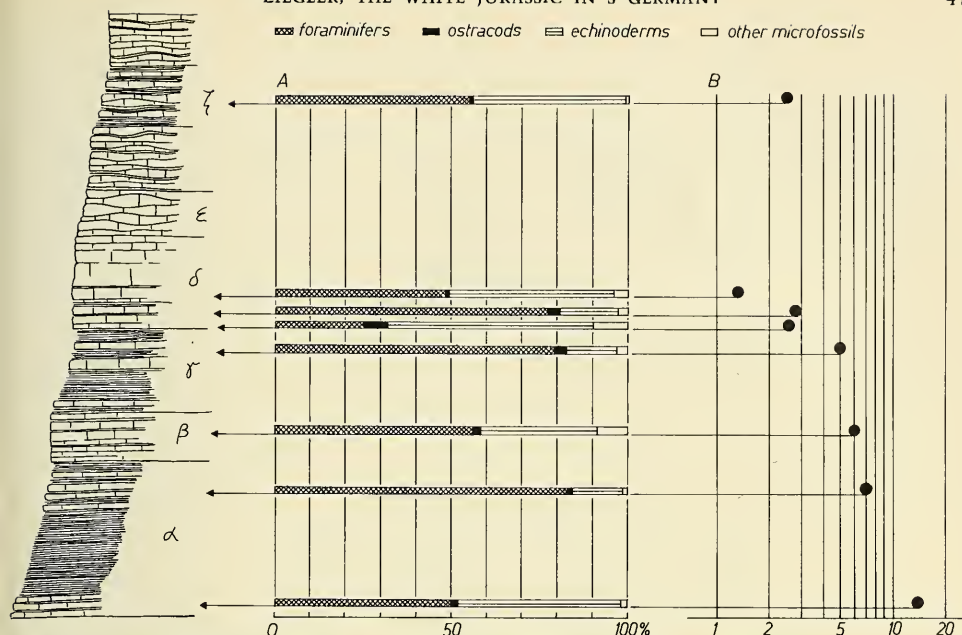
Fig. 36. The microfauna of marly sponge-algal sediments in the Swabian White Jurassic. After P. WAGENPLAST (1972).
