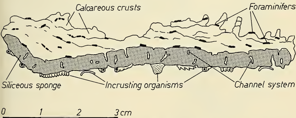
Fig. 24. Cross section through a siliceous sponge (dotted) covered by calcareous crusts and settled on its lower surface by sessile organisms. After G. K. FRITZ (1958).
