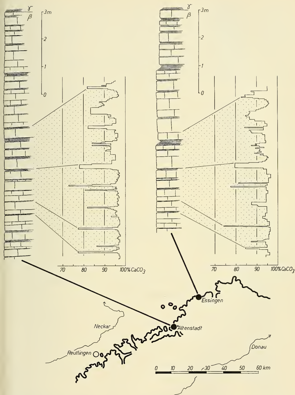
Fig. 21. Correlation of individual limestone beds over a distance of about 25 km in connection with the content of calcium carbonate. Upper part of the White Jurassic \beta of the eastern Swabian Alb. After H. WEILER (1957).
