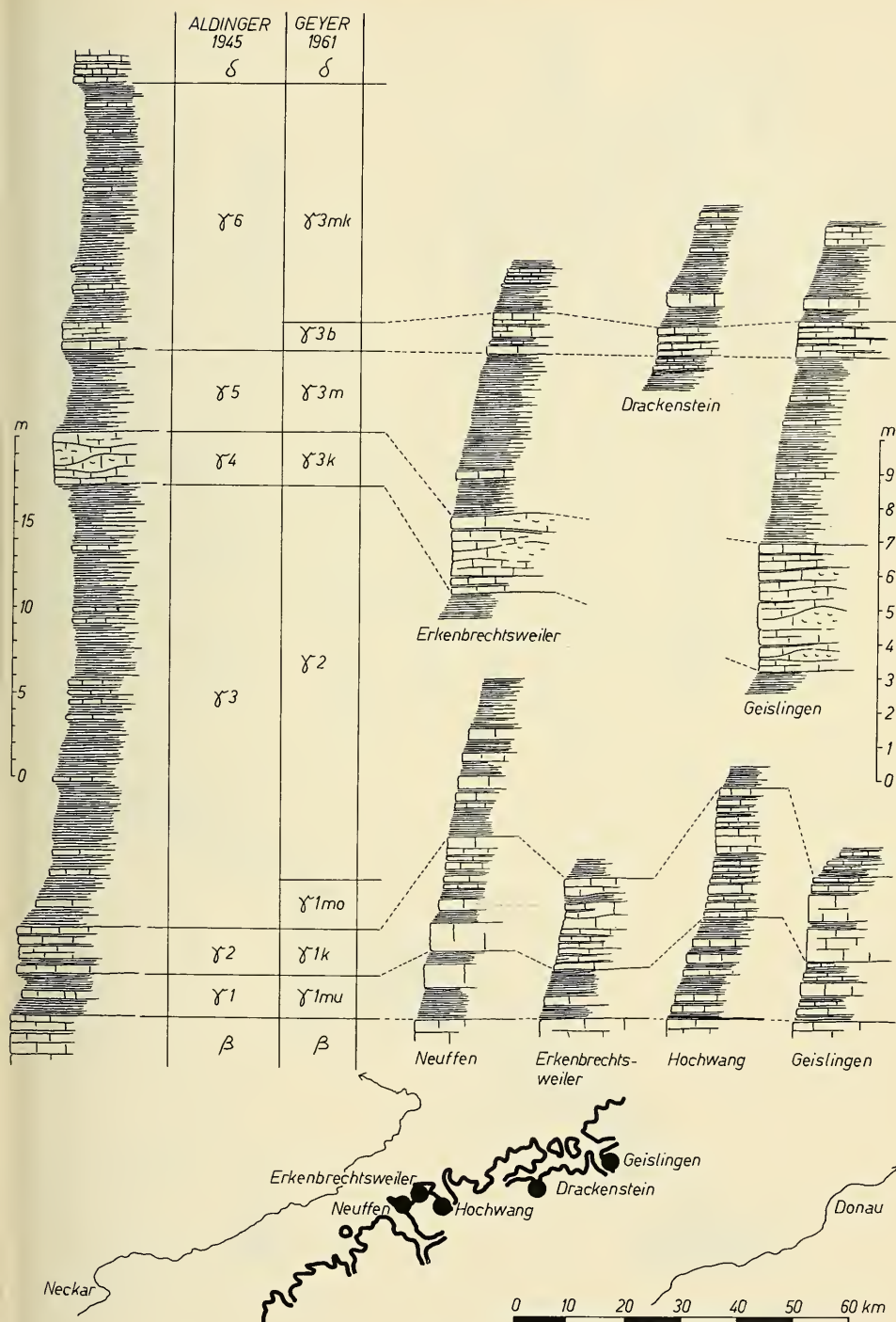
Fig. 7. The lithostratigraphy of the White Jurassic \gamma in the central part of the Swabian Alb. After H. ALDINGER (1945) and O. F. GEYER (1961 a).
