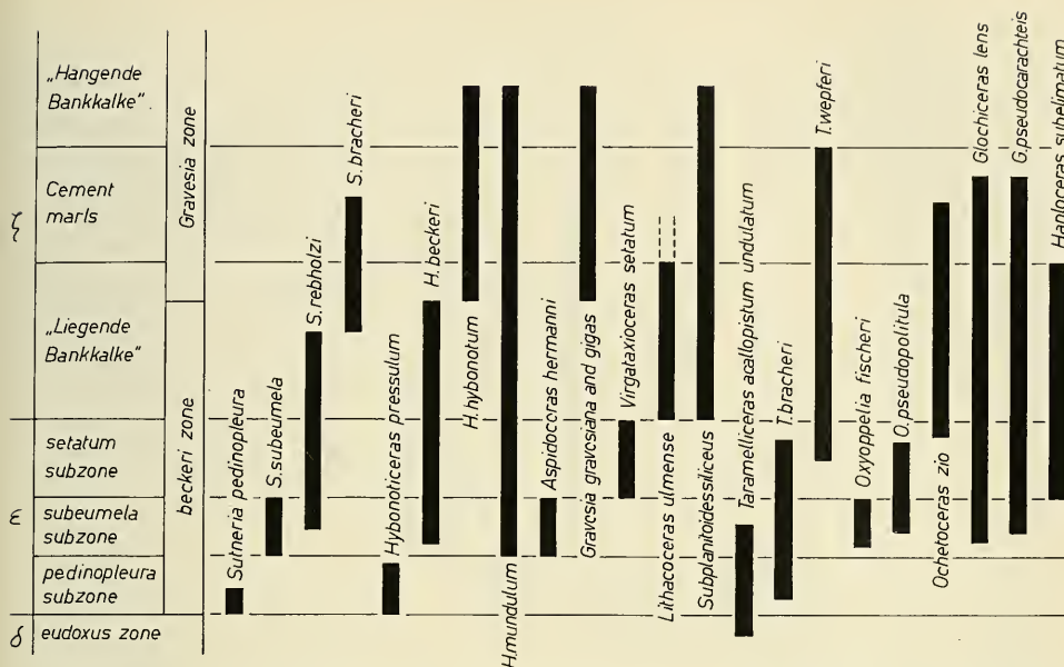
Fig. 19. Ranges of some ammonites in the White Jurassic ε and ζ in the Swabian Alb. Mainly after F. BERCKHEMER & H. HÖLDER (1959) and D. SEEGER (1961), slightly modified.
