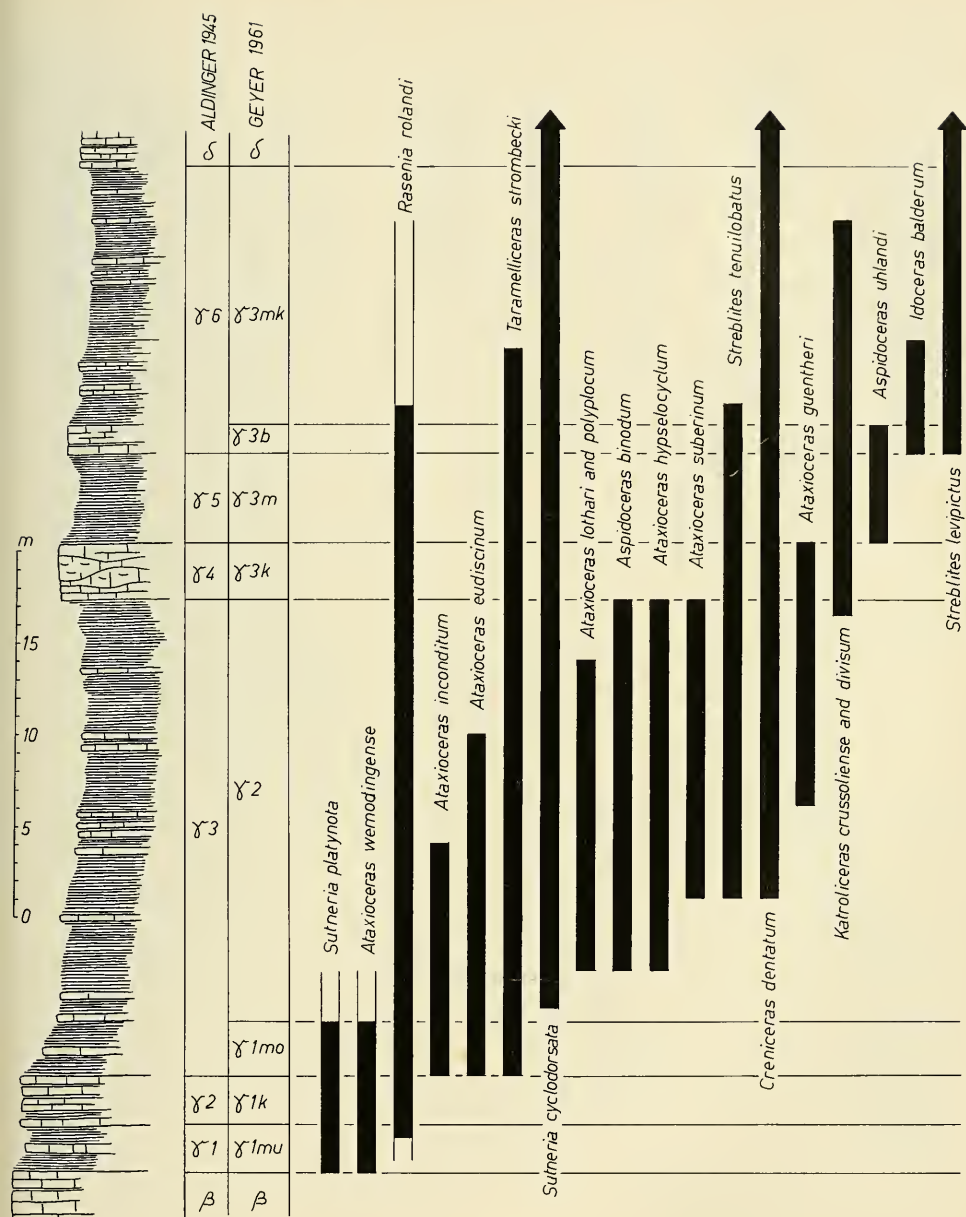
Fig. 17. Ranges of some ammonites in the White Jurassic γ in the Swabian Alb. Mainly after O. F. GEYER (1961 a; 1961 b).
