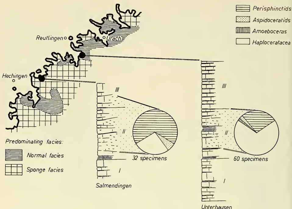
Fig. 35. The composition (according to individuals) of two ammonite faunas of the major ammonite groups. White Jurassic \delta 1 (lower acanthicum zone) of the central Swabian Alb. Salmendingen: Section with sponge-algal limestones within a region of predominant sponge facies.
