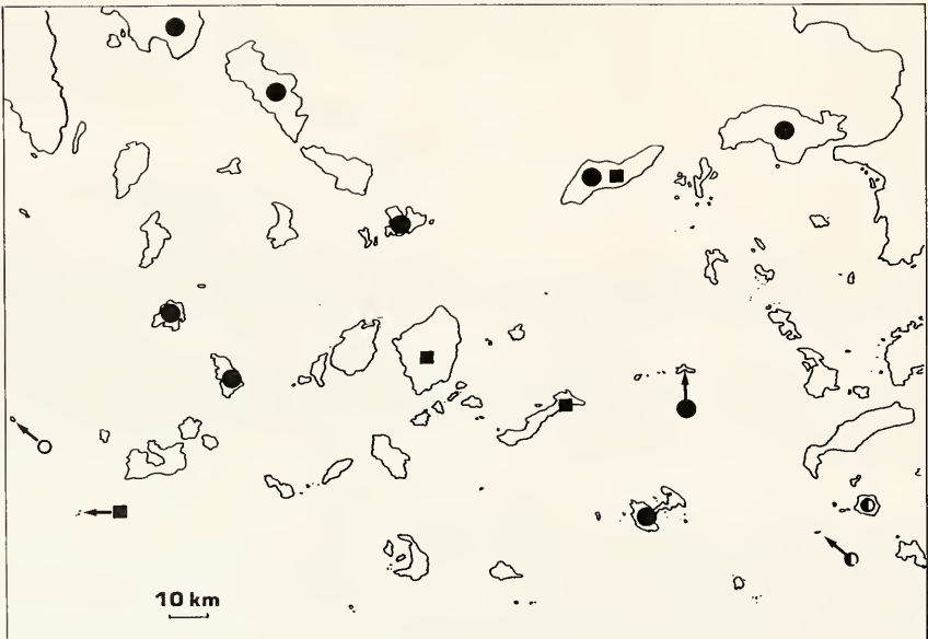
Fig. 60. The distribution of Trichoniscus oedipus (●), Parascbizidium album (■), P. falkoneriae (○) and P. polyvotisi (○).
