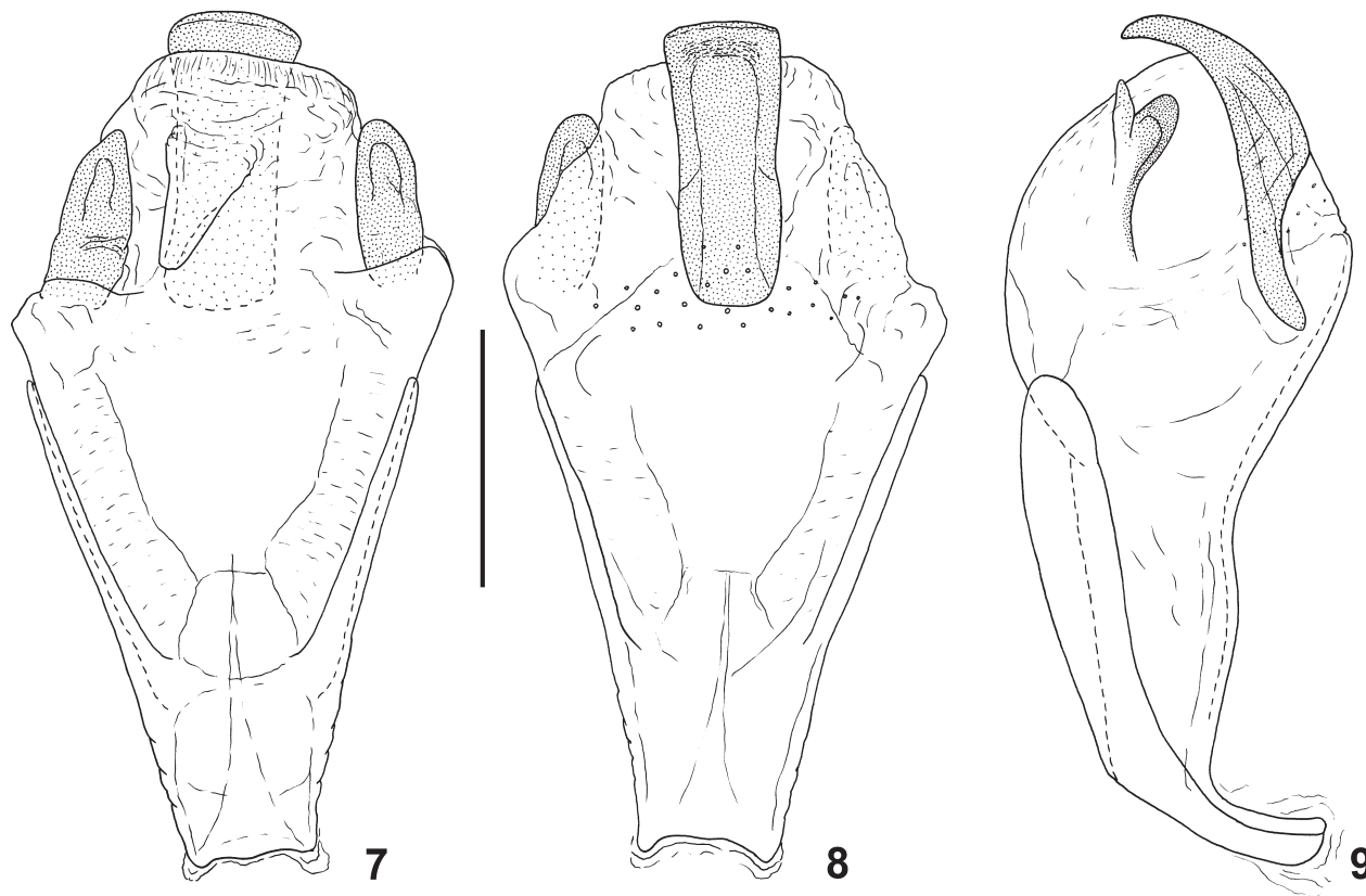
Figs. 7–9. Neuraphes qinghaiensis n. sp., aedeagus in dorsal (7), ventral (8), and lateral (9) views. – Scale: 0.1 mm.
