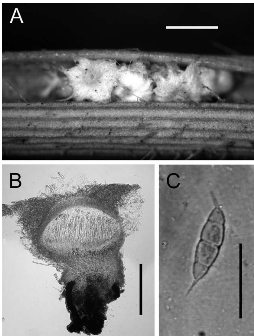
Fig. 1. Photographs of Puttemansia verrucosa (R. Kirschner & M. Piepenbring 1705; BPI 844025). A. Ascomata seen from above on the bamboo leaf. Scale bar = 500 \mu\text{m} . B. Longitudinal section of an ascoma. Scale bar = 250 \mu\text{m} . C. Ascospore (in 5 % KOH, phloxine). Scale bar = 25 \mu\text{m} .
