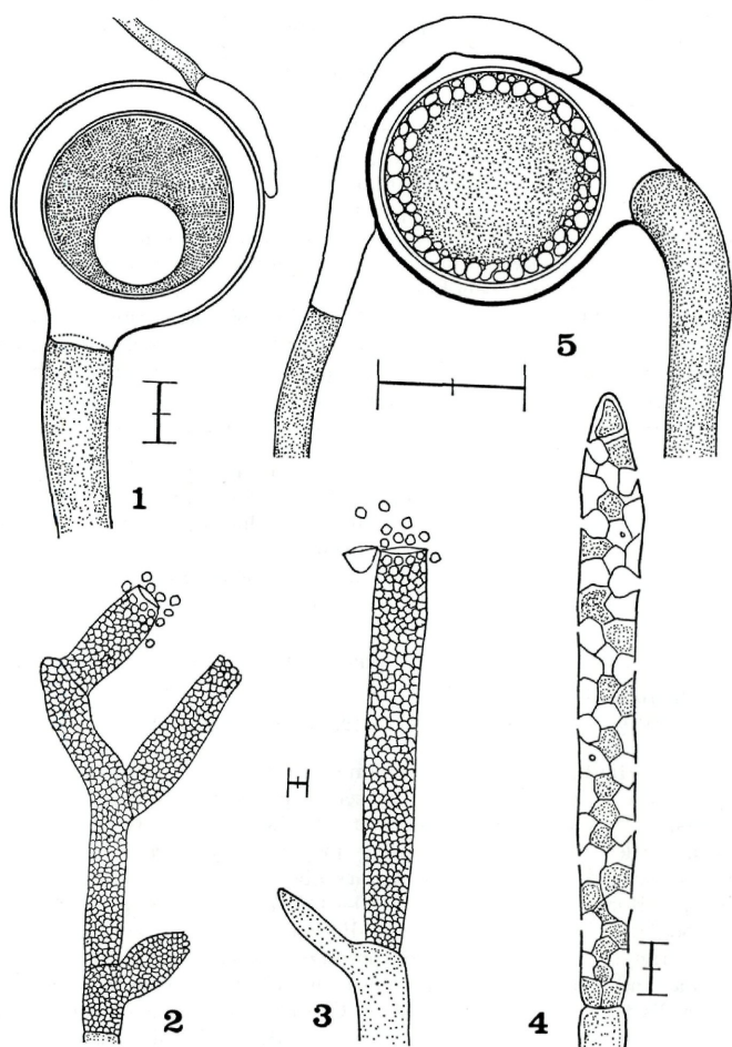
Figs. 1 – 5. Calyptralegnia ripariensis (1–3), 1, oogonium with eccentric oospores; 2, 3, zoosporangia showing discharge of zoospores. Dictyuchus pseudo-achlyoides (4–5), 4, zoosporangium true-net type; 5, oogonium with curved oogonial stalk. Scale, 20 \mu m
