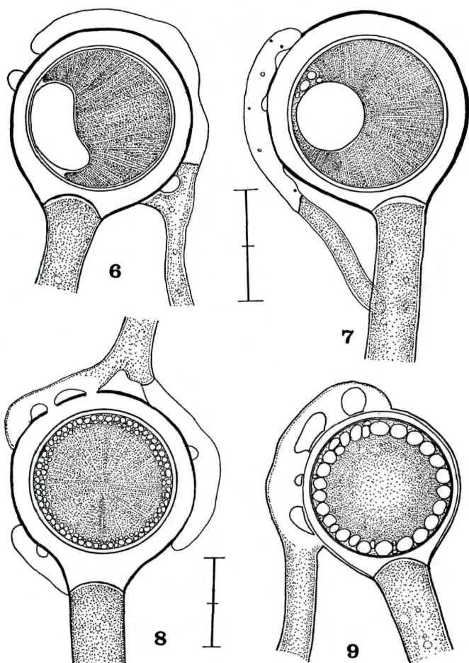
Figs. 6–9. Dictyuchus carpophorus (6–7), oögonia each with a single eccentric oospore. Dictyuchus monosporus (8–9), oögonia each with a single centric oospore. Scale, 20 µm
