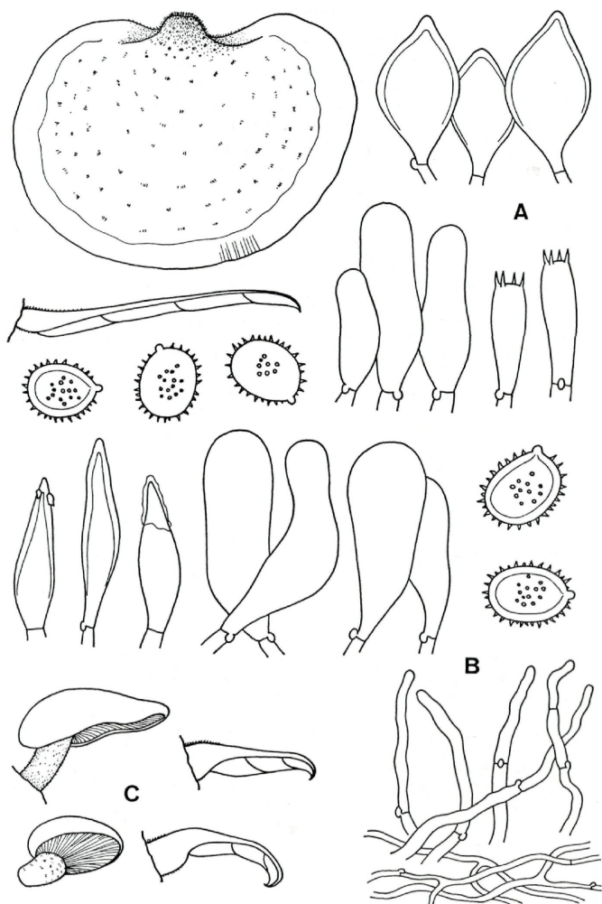
Fig. 3. Conchomyces bursaeformis (BERK.) H.K.: A. carpophores, spores, cheilocystidia, pleurocystidia (ZT, 72/260). — B. spores, cheilocystidia, pleurocystidia, cuticle of pileus (ZT, 75/281). — C. carpophores (ZT, 62/210)
