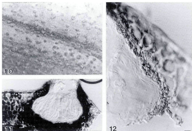
Figs. 10–12. – Carinispora nypae . – 10. Appearance of ascomata on host surface. – 11. Section of ascma. – 12. Peridium. – Bars: 10 = 500 \mu\text{m} , 11 = 100 \mu\text{m} , 12 = 10 \mu\text{m} .
