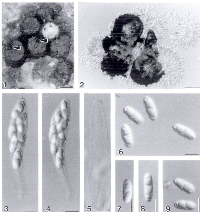
Figs. 1–9. – Interference contrast micrographs of Aniptodera nypae . – 1. Ascus immersed in old fruiting bodies of Linocarpon sp. (arrowed). – 2. Squash illustrating ascomata. – 3–5. Asci. Note the apical refractive thickening and pore. – 6–9. Ascospores. – Bars: 1 = 500 \mu\text{m} , 2 = 100 \mu\text{m} , 3–9 = 10 \mu\text{m} .
