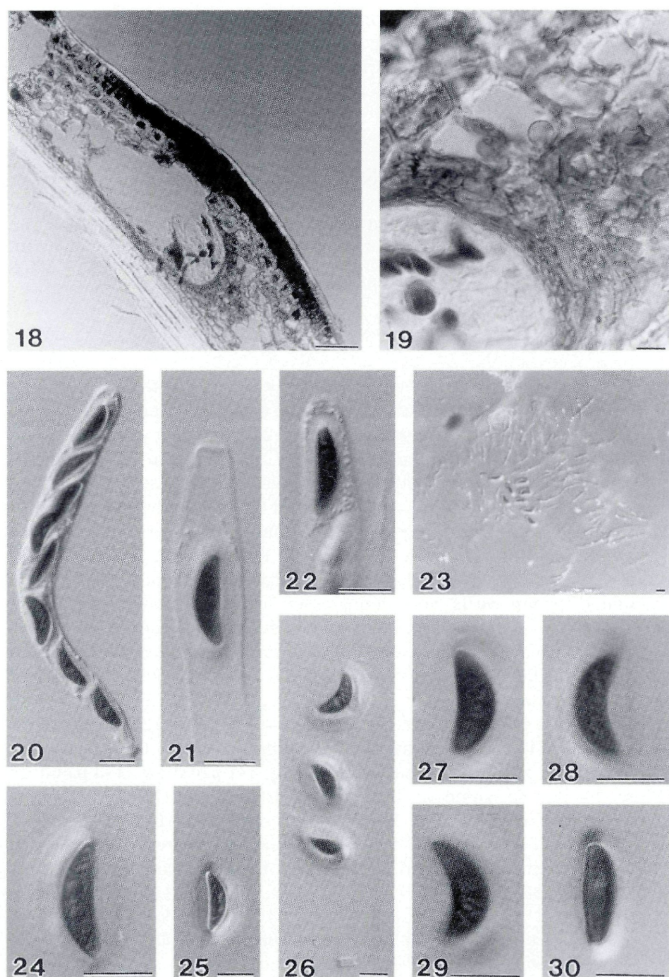
Figs. 18–30. – Interference contrast micrographs of Nipicola selangorensis . – 18. Section of ascus. – 19. Peridium. – 20–22. Asci. Note the lightly staining ring. – 23. Amphisphaeriaceous paraphyses. – 24–30. Ascospores with layered sheath (24–28) and germ slit (30). – Bars: 18 = 100 \mu\text{m} , 19–30 = 10 \mu\text{m} .
