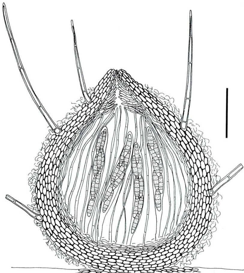
Fig. 8. Chaetosphaeria exserticlavoides . – Median longitudinal section of the perithecium. – Scale bar = 50 \mu m. From PRM 900540 (Holotype).
