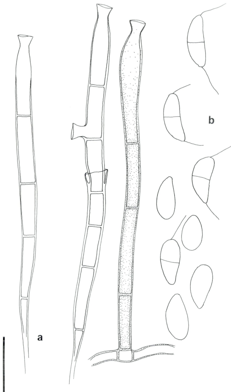
Fig. 17a, b. Chaetosphaeria falacrospora . – a. Conidiophores of the Dictyochaeta anamorph. – b. Conidia. – Scale bar = 10 \mu m. – From culture CBS 112962 ex PRM 900541.
