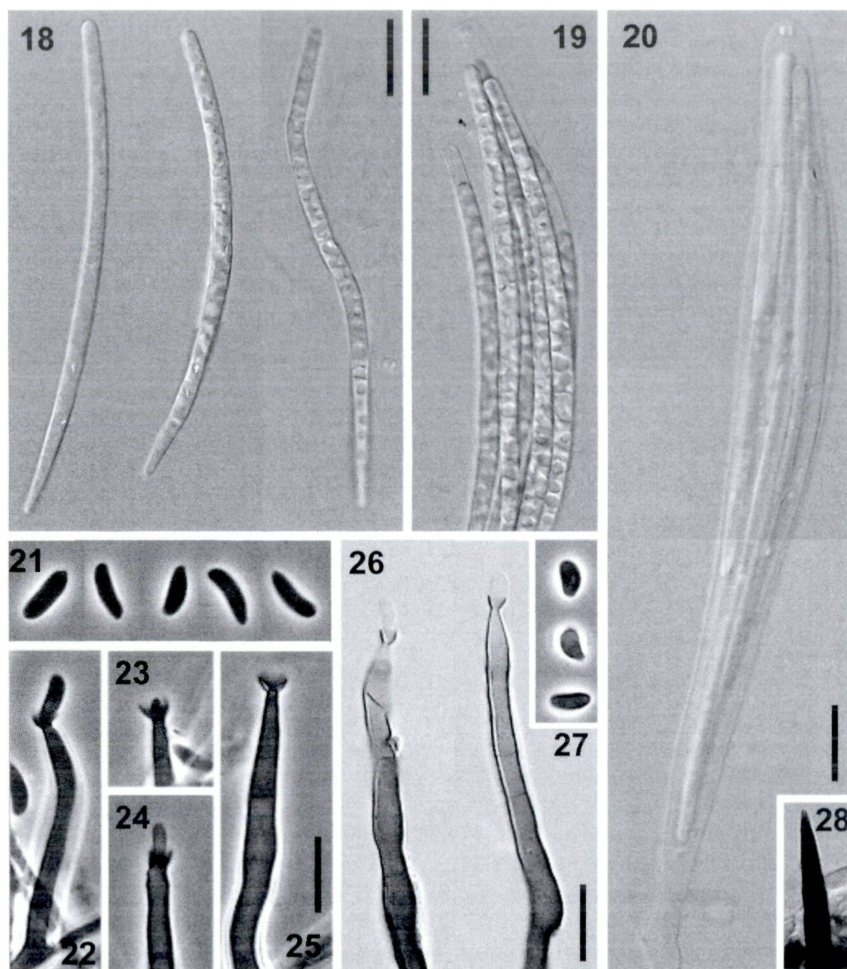
Figs. 18–28. Chaetosphaeria hispida . – 18. Ascospores. – 19. Upper part of ascus containing apical annulus. – 20. Ascus. – 21. Conidia of the Dictyochoaeta anamorph. – 22–26. Conidiophores and conidiogenous cells. – 27. Conidia. – 28. Perithecial seta. – Scale bar = 10 \mu\text{m} . – Figs. 18–20, 26, 28: DIC; 21–25, 27: PC. – Figs. 18–28 from PRM 900543 (Holotype); 21–25 from culture CBS 112964; 26, 27 from nature.
