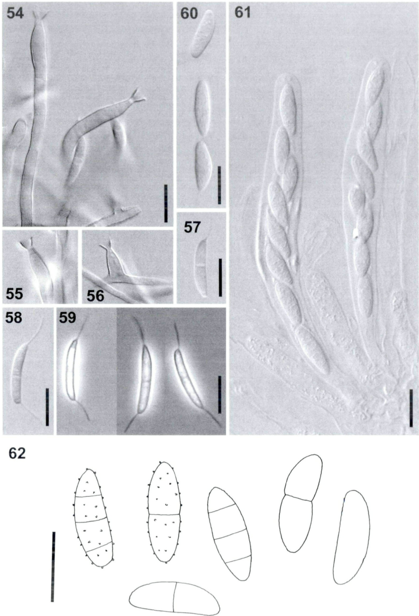
Figs. 54–62. Chaetosphaeria verruculospora . – 54–56. Conidiophores and conidio-genous cells of the Codinaea anamorph. – 57–59. Conidia. – 60. Ascospores. – 61. Asci containing ascospores. – 62. Ascospores. – Scale bar = 10 µm. – Figs. 54–58, 60, 61: DIC; 59: PC. – Figs. 54–62 from PRM 900542 (Holotype); 54–59 from culture.
