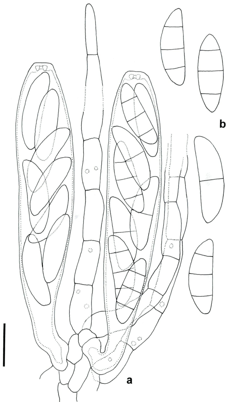
Fig. 53a, b. Chaetosphaeria tubulicollaris . – a. Asci with ascospores and paraphyses. – b. Ascospores. – Scale bar = 10 µm. From PRM 900545 (Holotype).
