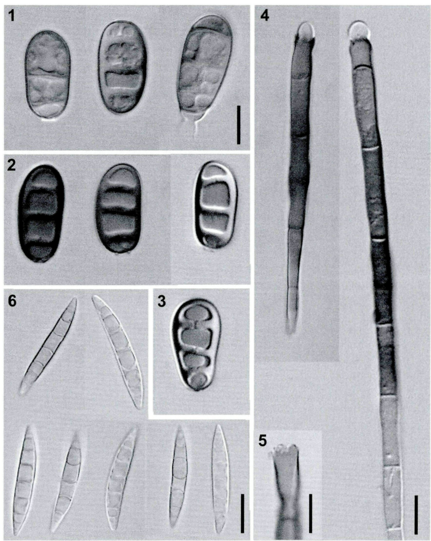
Figs. 1–6. Chaetosphaeria exserticlavoides . – 1–3. Conidia of the Exserticlava anamorph. – 4, 5. Conidiophores. – 6. Ascospores. – Scale bar = 10 µm. – Figs. 1–6: DIC. – Figs. 1–6 from culture CBS 112963 ex PRM 900540 (Holotype).
