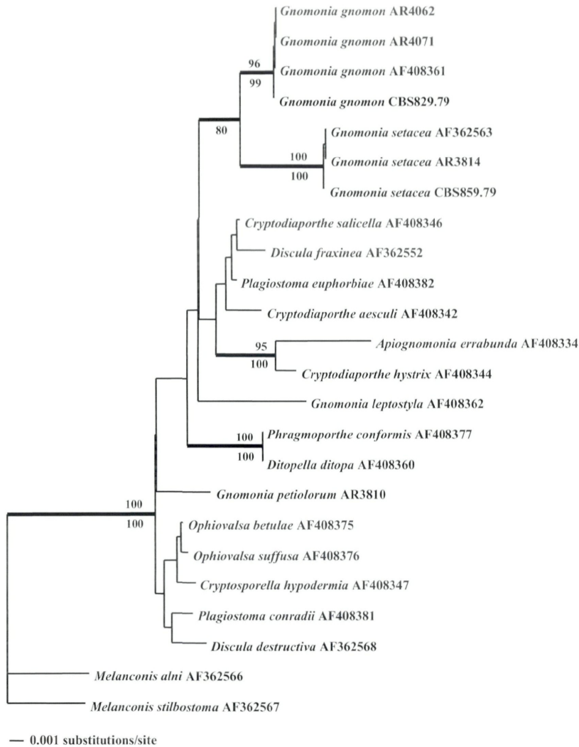
Fig. 19. – Phylogenetic tree resulting from Neighbor-Joining analysis of 1302 bp of the nLSU rDNA sequences of 22 strains representing the Gnomoniaceae. Bootstrap values greater than 70 % are shown above (based on maximum parsimony analysis) and below (NJ) each branch. Thickened lines indicate that branch appeared in the strict consensus of the 386 trees resulting from maximum parsimony analysis (length = 117, CI = 0.650, RI = 0.785, RC = 0.510).
