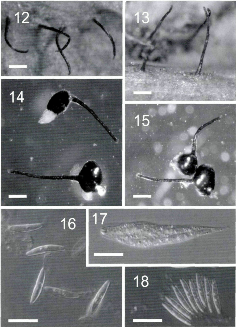
Figs. 12–18. Gnomonia setacea . 12, 13. Dried perithecia on natural substrata. – 14, 15. Rehydrated perithecia from natural substrata. – 16, 18. Ascospores. – 17. Ascus. – Figs. 12, 14, 16. Deutschl. Schw. 132. – 13. BPI 844268. – 15, 17, 18. BPI 844261. – Figs. 12–15. Dissecting microscope. – 16–19. DIC. – Scale bars: 12–15 = 200 \mu m; 16–18 = 10 \mu m.
