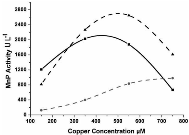
Fig. 4. Manganese peroxidase production by (—■—) Ganoderma stipitatum , (---●---) Lentinus crinitus , (---▲---) Lentinus swartzii , at different Cu^{2+} concentrations under submerged cultivation at 30 °C and 20 th day of cultivation.
