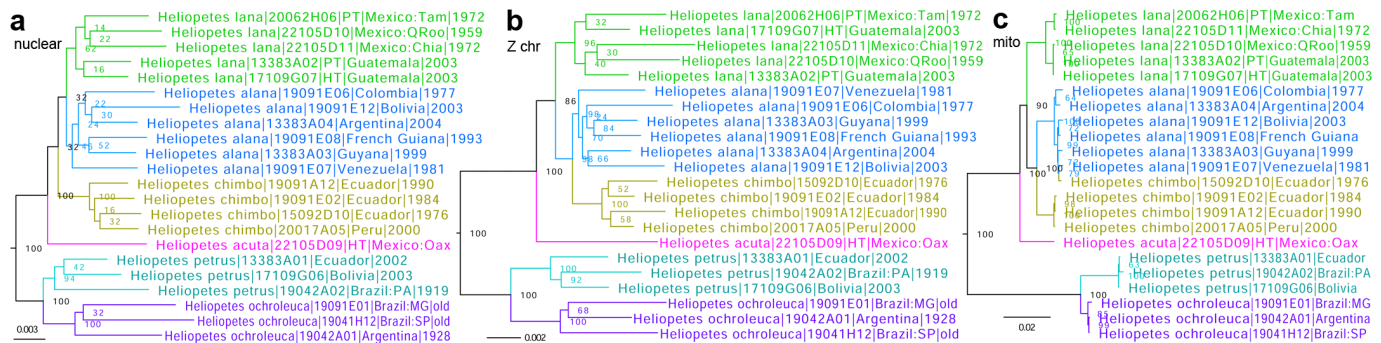
Fig. 24. Phylogenetic trees of selected Heliopetes (Heliopetes) species inferred from protein-coding regions of a) the nuclear genome (autosomes), b) the Z chromosome, and c) the mitochondrial genome. Different species are shown in different colors: H. lana (green), H. alana (blue), H. chimbo (olive), H. acuta sp. n. (magenta), H. petrus (Hübner, [1819]) (cyan), and H. ochroleuca J. Zikán, 1938 (purple). Note the introgression of H. alana mitochondrial DNA into one H. chimbo specimen (NVG-15092D10).
