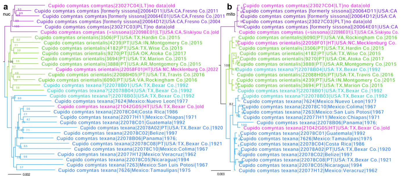
Fig. 20. Phylogenetic trees of Cupido comyntas subspecies inferred from protein-coding regions of a) the nuclear (autosomes) and b) the mitochondrial genome. Different subspecies are shown in different colors (primary types are labeled in magenta): C. comyntas comyntas (purple, including Lycaena sissona W. G. Wright, 1905 as its synonym), C. comyntas orientalis ssp. n. (green), and C. comyntas texana (blue). Specimens more recently collected near the type locality of C. comyntas texana are labeled in cyan.
