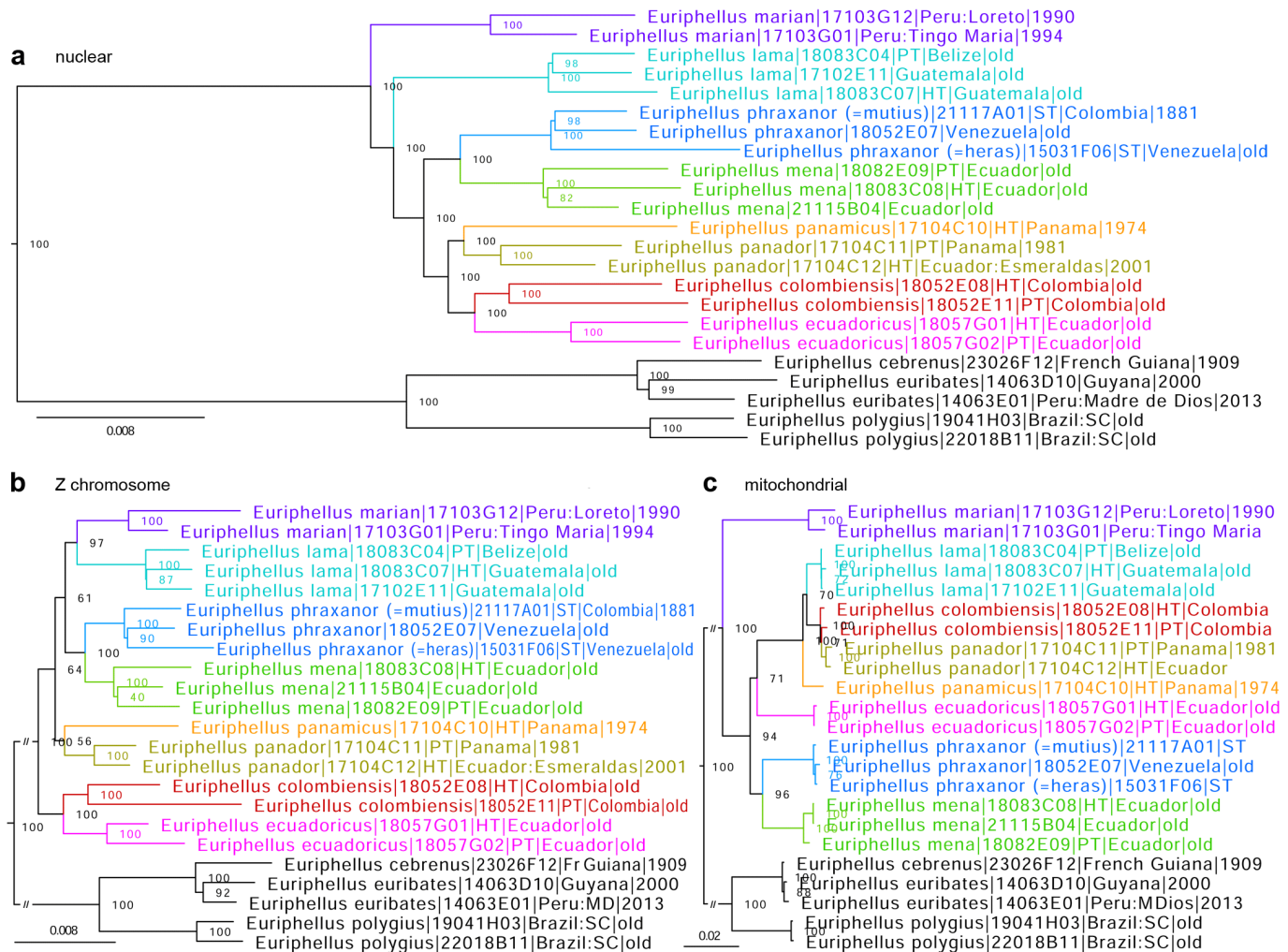
Fig. 23. Phylogenetic trees of all described Euriphellus species inferred from protein-coding regions of a) the nuclear genome (autosomes, about 3 million positions and ultrafast bootstrap (Minh et al. 2013) were used), b) the Z chromosome, and c) the mitochondrial genome. Different species of the E. phraxanor group are colored differently: E. marian (violet), E. lama (cyan), E. phraxanor (blue), E. mena (green), E. panamicus (orange), E. panador (olive), E. colombiensis sp. n. (red), and E. ecuadoricus sp. n. (magenta). Sections of the Z chromosome and mitogenome trees corresponding to long branches were removed (as indicated by //) to fit in the allotted space.
