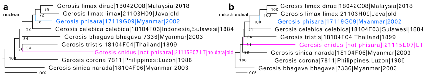
Fig. 27. Phylogenetic trees of selected Gerosia species inferred from protein-coding regions of a ) the nuclear (autosomes) and b ) the mitochondrial genome: Gerosia phisara (blue) and Gerosia cnidus stat. rest. (magenta).
