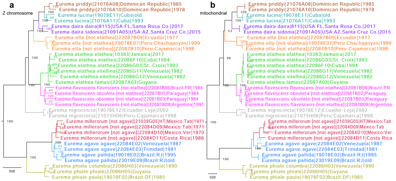
Fig. 3. Phylogenetic trees of all known species of Eurema inferred from protein-coding regions of a) the Z chromosome (best for species delineation) and b) the mitochondrial genome. Different species are colored differently: E. priddy (Lathy, 1898) (brown), E. lucina (Poey, [1852]) (cyan), E. दौर (purple), E. ella stat. nov. (orange), E. elathea (green), E. flavescens (Chavannes, 1850), stat. rest. (magenta), E. nigrocincta Dognin, 1889 (gray), E. millerorum stat. nov. (red), E. agave (blue), and E. phiale (Cramer, 1775) (olive).
