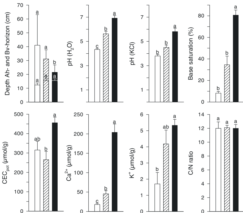
Fig. 10: Soil conditions in the Ah horizon of the Polytricho-Festucetum tenuifoliae / Galio-Deschampsietum flexuosae (white bars; n = 3 ), Festuco-Genistelletum (striped bars; n = 8 ) and Gentiano-Koelerietum (black bars; n = 10 ) in the lower Aar valley. Mean values and standard errors are shown. Values with different letters differ significantly at p < 0.05 . (see also Table 6)
