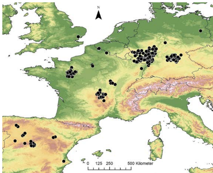
Fig. 5. Records of Epilobium brachycarpum in Europe during 1978–2011.
