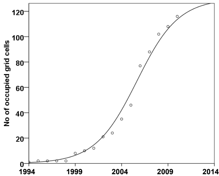
Fig. 3. The cumulative number of grid records (approx. 12 \times 11 km) for Epilobium brachycarpum in Germany during 1994–2010 (dots) can be described by a logistic growth function ( R^2 = 0.98 ).
