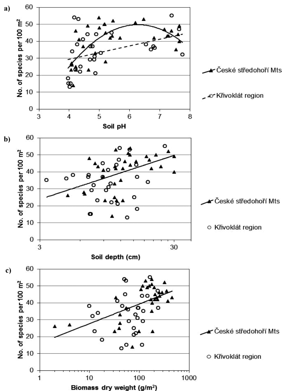
Fig. 4. Number of all vascular plant species recorded in dry grassland plots of 100 m² plotted against soil pH (a), soil depth (b) and productivity expressed as above-ground biomass dry weight without litter (c). Lines are fitted for significant ( P < 0.05 ) regressions only: non-significant relationships for the Křivoklát region in (b) and (c) are not shown.
