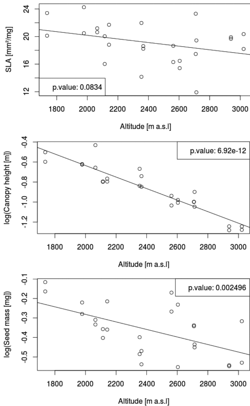
Fig. 7. Community-weighted means of the “Westoby traits” L (specific leaf area, SLA; R^2 = 0.08 ), H (canopy height; R^2 = 0.86 ) and S (seed mass; R^2 = 0.29 ) and their relation to elevation assessed with linear regression.
