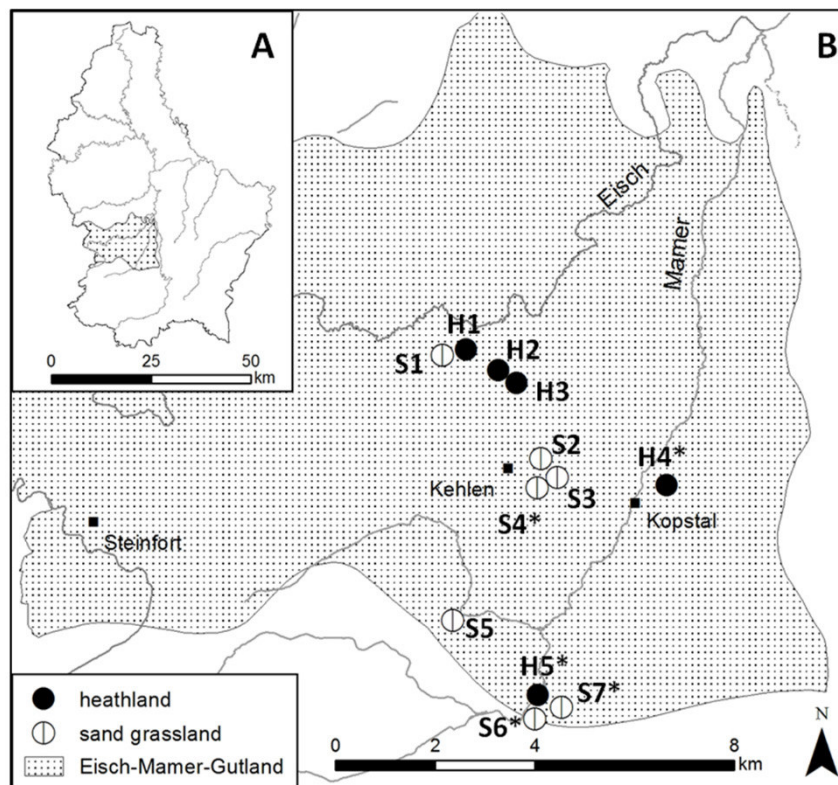
Fig. 1. Map of the study area “Eisch-Mamer Gutland” in the southwest of Luxembourg A) and the location of the study sites B) . “H” is the abbreviation for heathland and “S” for sand grassland. New sites are marked with *. These sites have been restored less than 10 years ago. The other heathland and sand grassland sites have been restored over 10 years ago or are a result of long-lasting extensive management. (Source of the digital data base: ADMINISTRATION DU CADASTRE ET DE LA TOPOGRAPHIE LUXEMBOURG 2000).
