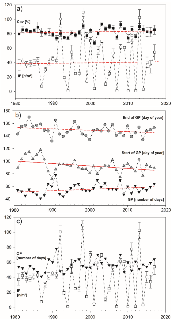
Fig. 2. Long-term dynamics of A. ursinum (1981 to 2017): a) inflorescence numbers (IF in n/m^2 ; white quadrates) and cover (Cov in %, black quadrates), b) start (grey triangles), end (grey circles) and length of the growing period (GP; black triangles), and c) inflorescence numbers (white quadrates) directly contrasted to the growing period (black triangles). IF and Cov are mean values of a different amount of 1 m^2 plots during the observation period. Error bars represent standard error, red lines the calculated Sen slope. The solid line shows a significant trend (see text for numbers).
