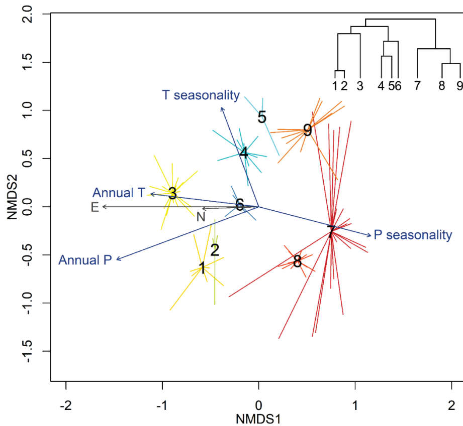
Fig. 3. NMDS analysis of the dataset with relev -to-cluster assignment and centroids of the clusters based on the classification analysis (see dendrogram in the right upper part). Vectors of geographical position (in black) and climatic variables (in blue) were passively plotted. Stress value = 0.214.
