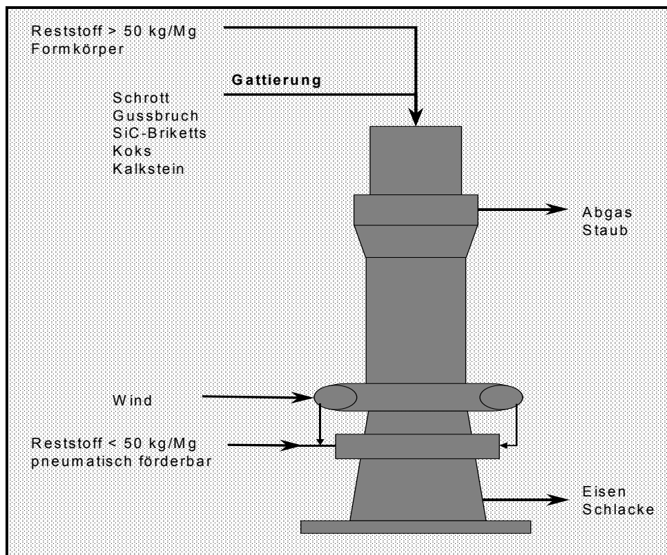
Abb. 3-11: Kupolofen
