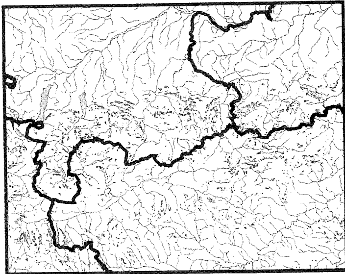
min - Operator
