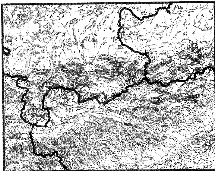
max - Operator
