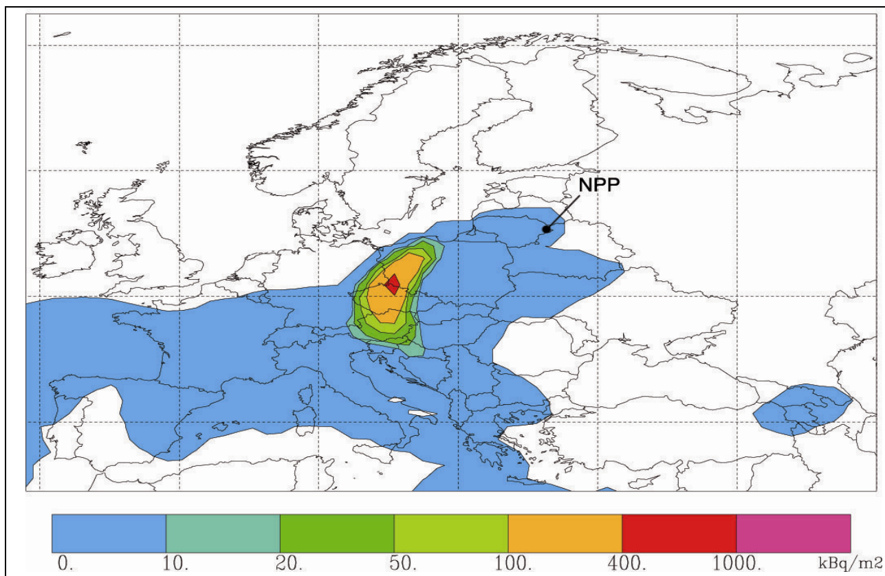
Figure 2: Example of deposition of Cs-137 over Europe resulting from a hypothetical severe accident in the new Ignalina NPP, assuming a release of 35.5 PBq in the hour after 1995-06-25 14:56. Output grid size is 1°. The outer border of the blue colour is at 0.1 kBq/m 2 .
